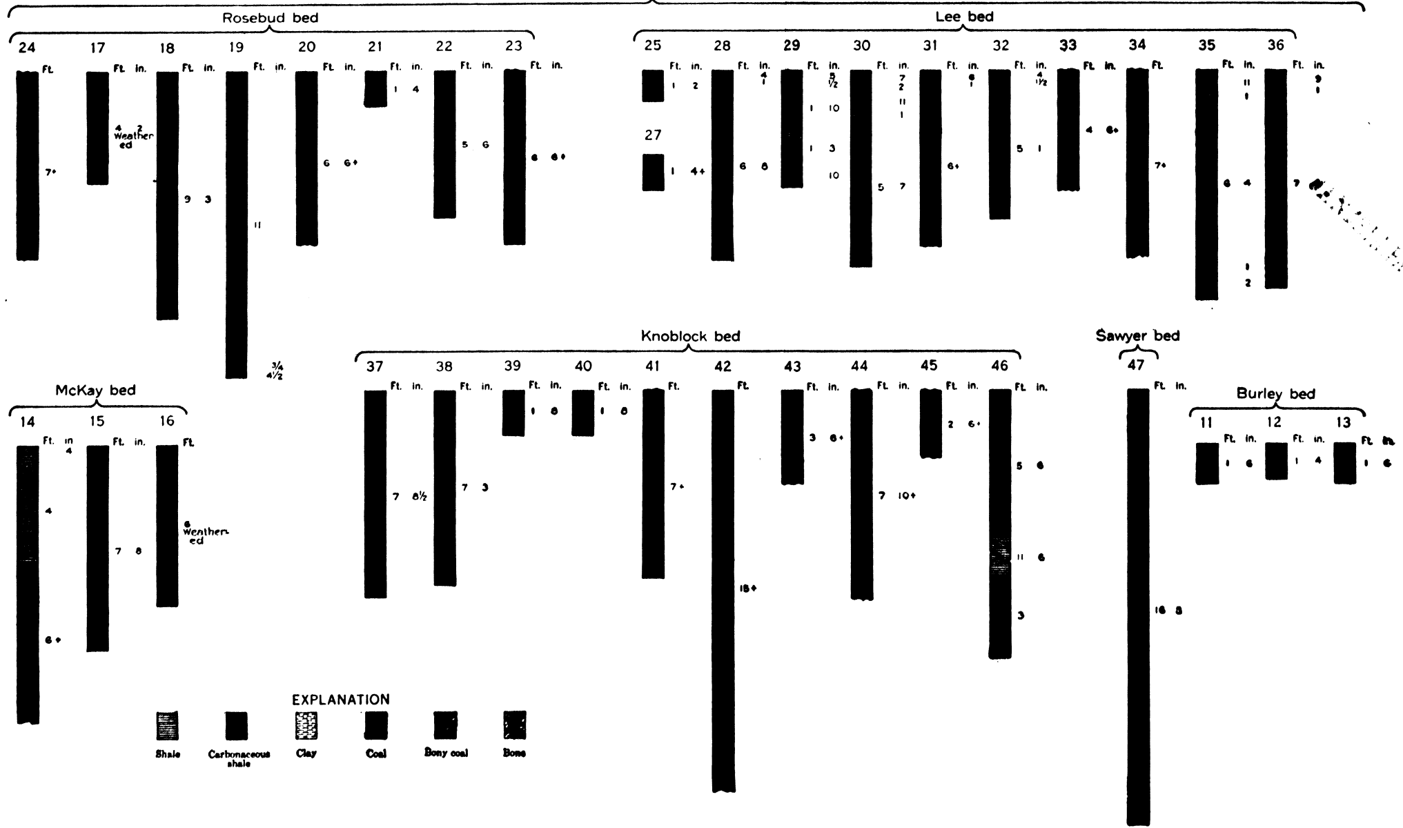
COAL SECTIONS IN ASHLAND FIELD
