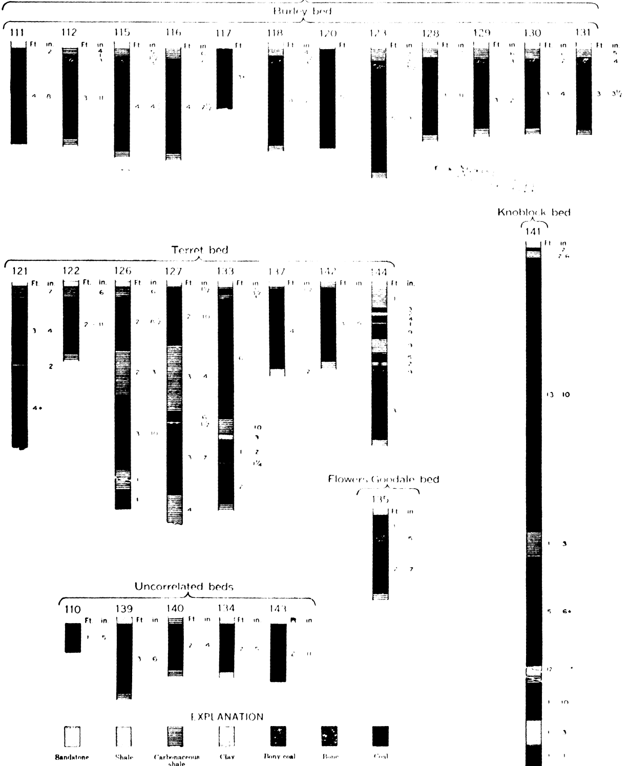
COAL SECTIONS IN ASHLAND FIELD
