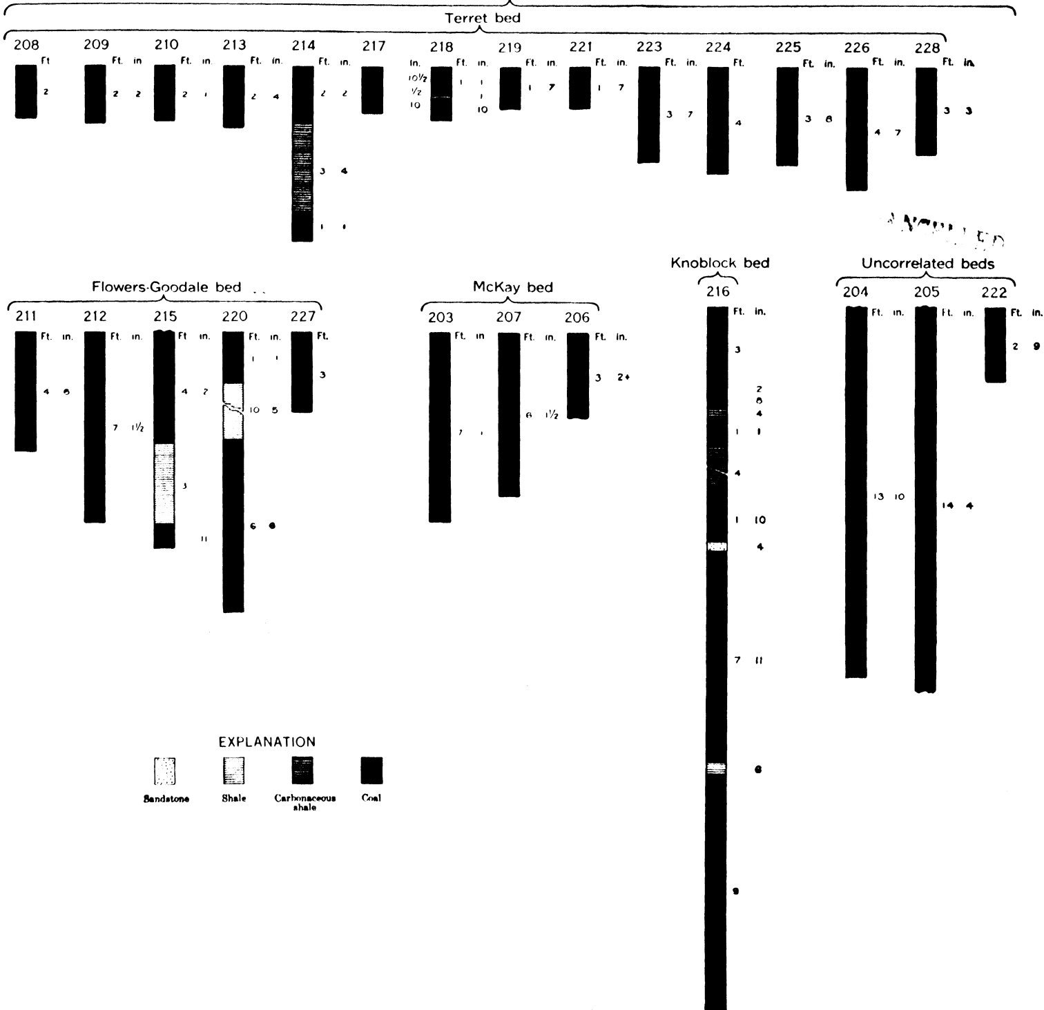
COAL SECTIONS IN ASHLAND FIELD
