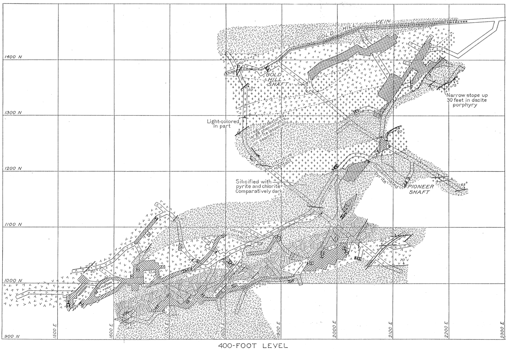
GEOLOGIC MAPS OF THE 250, 400, AND 700 LEVELS, GOLD HILL MINE.
