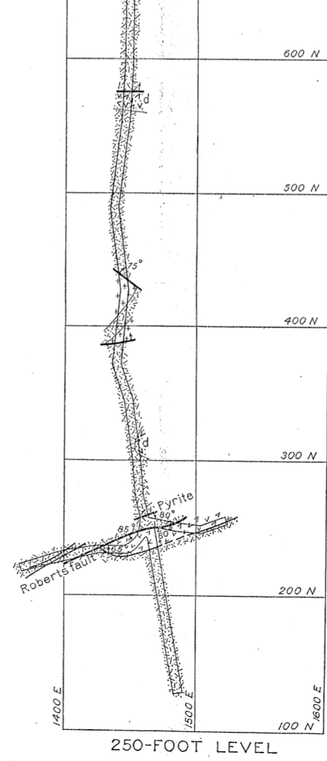
GEOLOGIC MAPS OF THE 250, 400, AND 700 LEVELS, GOLD HILL MINE.
