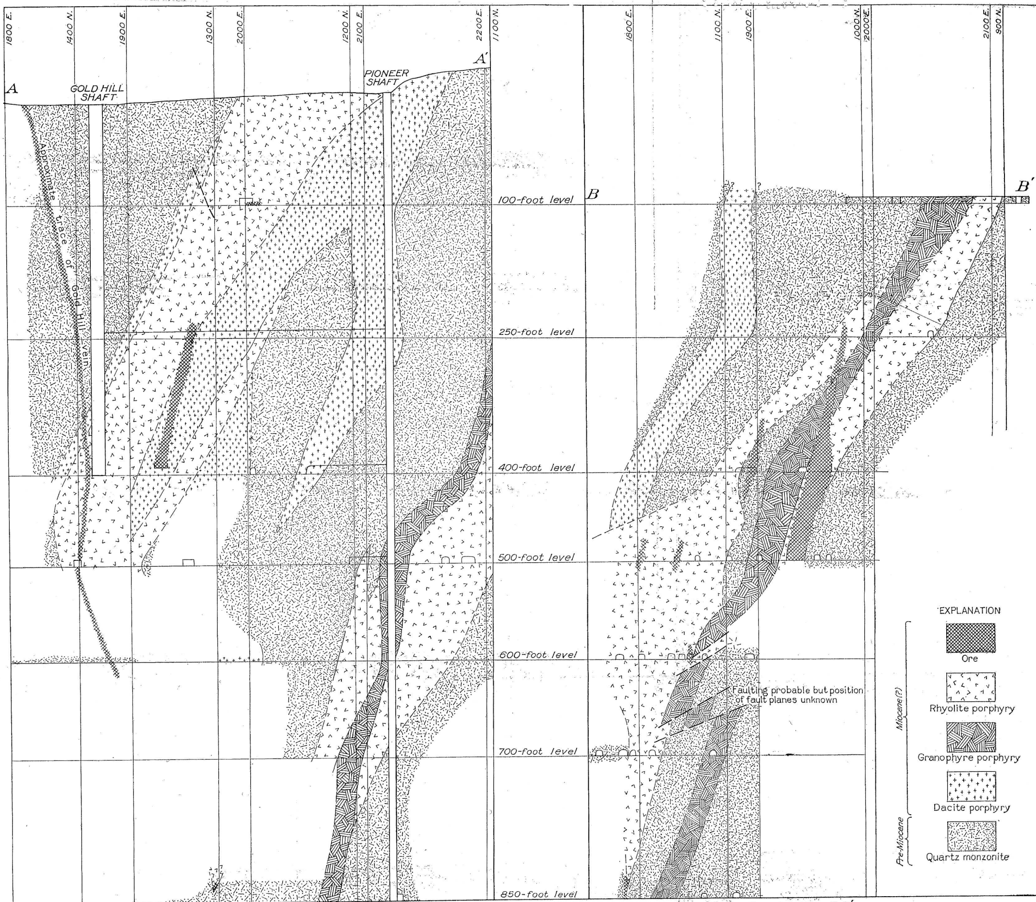
DIAGRAMMATIC GEOLOGIC SECTIONS THROUGH THE GOLD HILL MINE.
