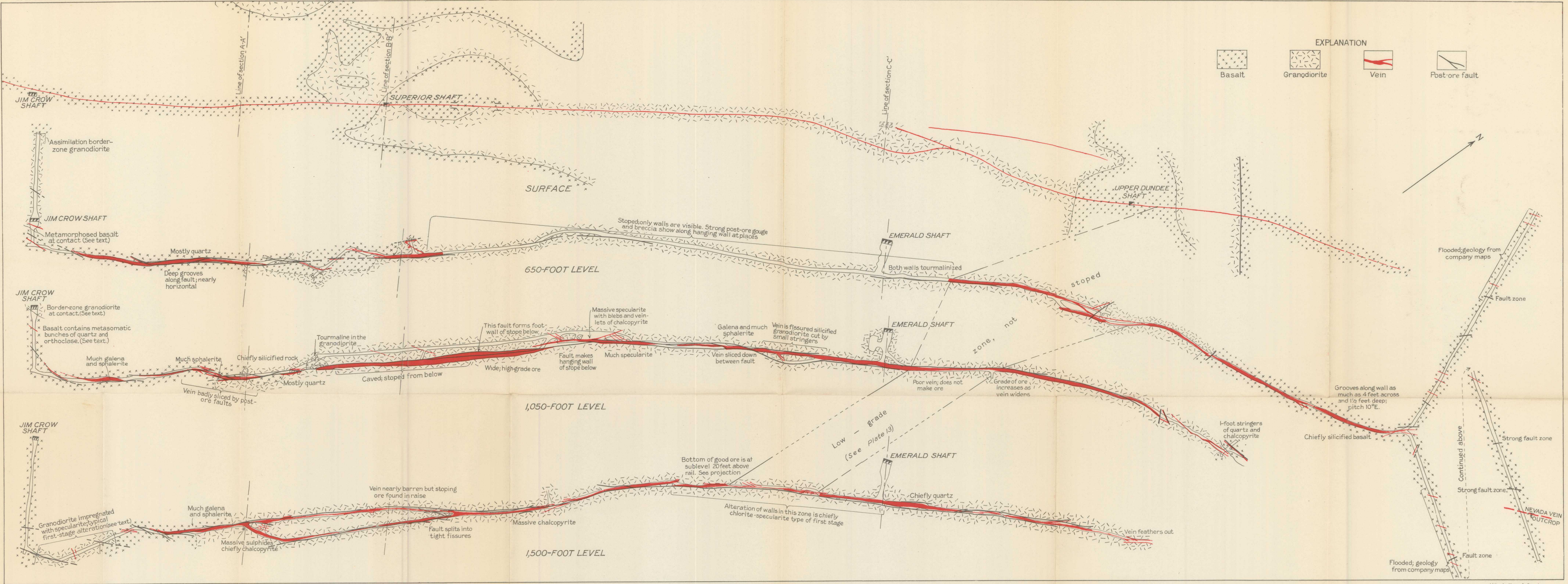
GEOLOGIC PLANS OF THE 650-, 1050-, AND 1500-FOOT LEVELS OF THE EIGHTY-FIVE MINE AND SURFACE GEOLOGY ALONG THE OUTCROP
