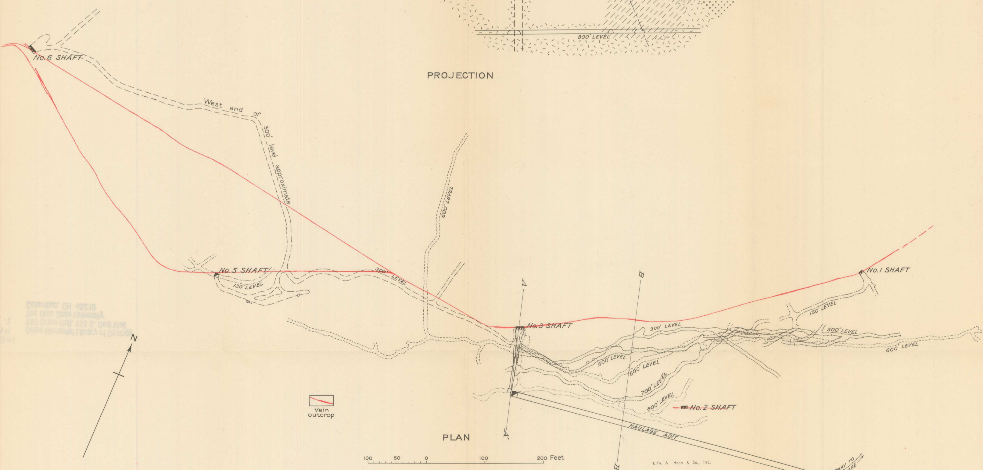
PLAN AND PROJECTION OF THE ANITA MINE
