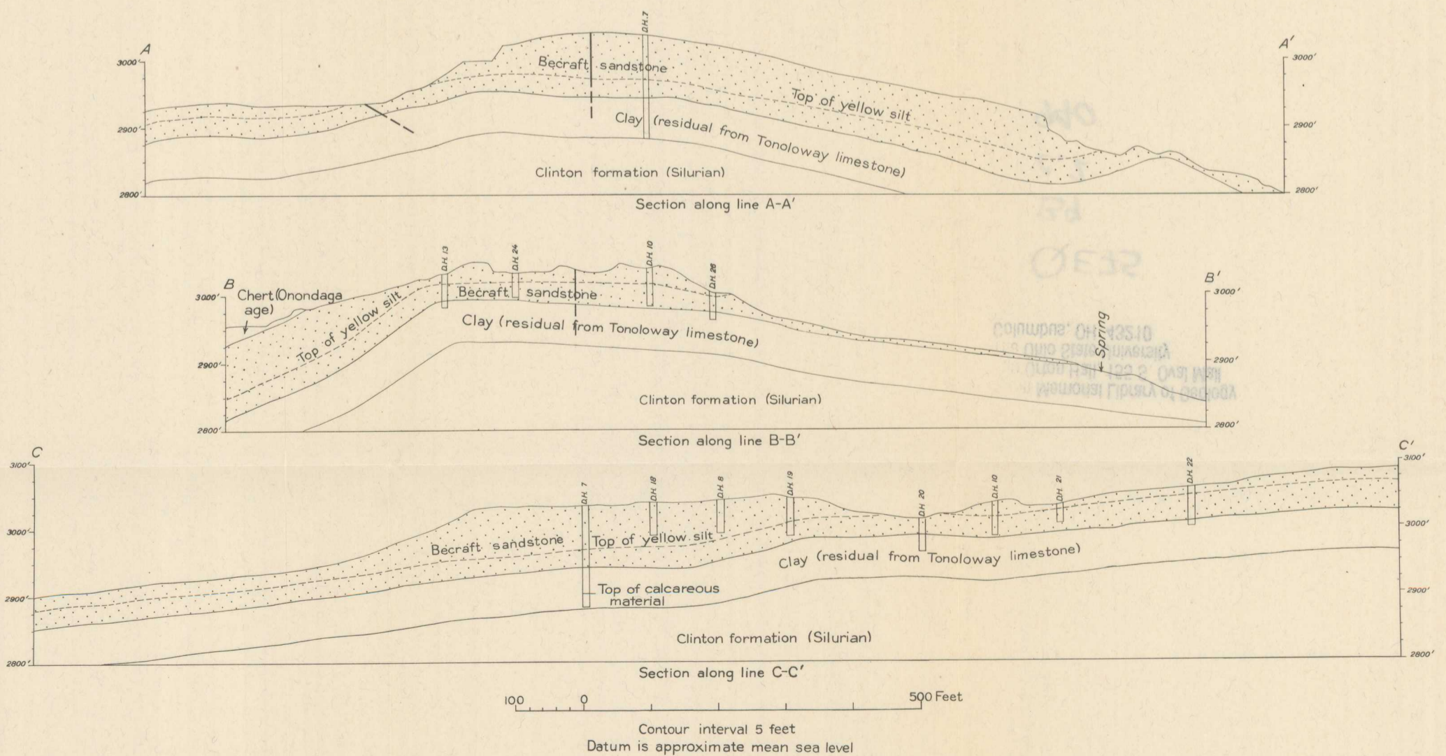
MAP AND SECTIONS OF STANGE AND ARMS MINES, BLAND COUNTY, VIRGINIA
