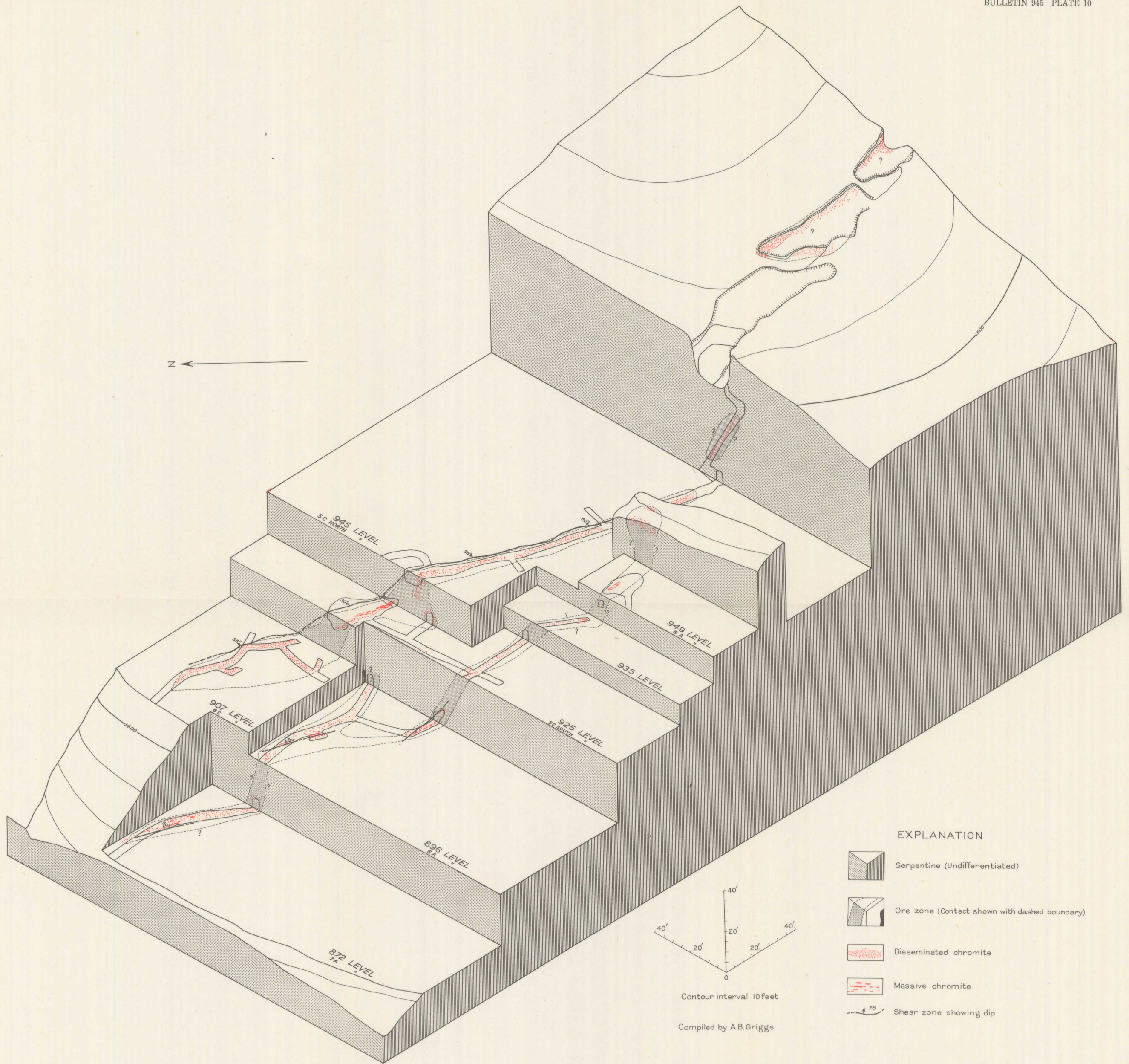
BLOCK DIAGRAM OF THE SWEETWATER MINE, SAN LUIS OBISPO COUNTY, CALIF.
