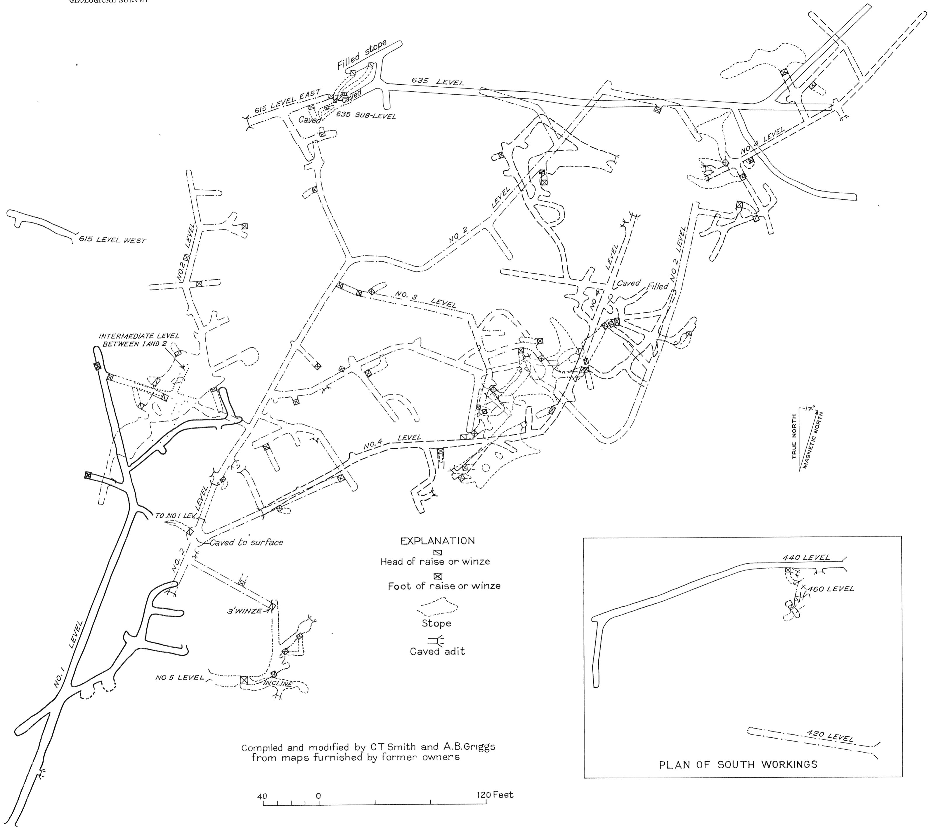
PLAN OF THE WORKINGS OF THE PICK AND SHOVEL MINE, SAN LUIS OBISPO COUNTY, CALIF.
