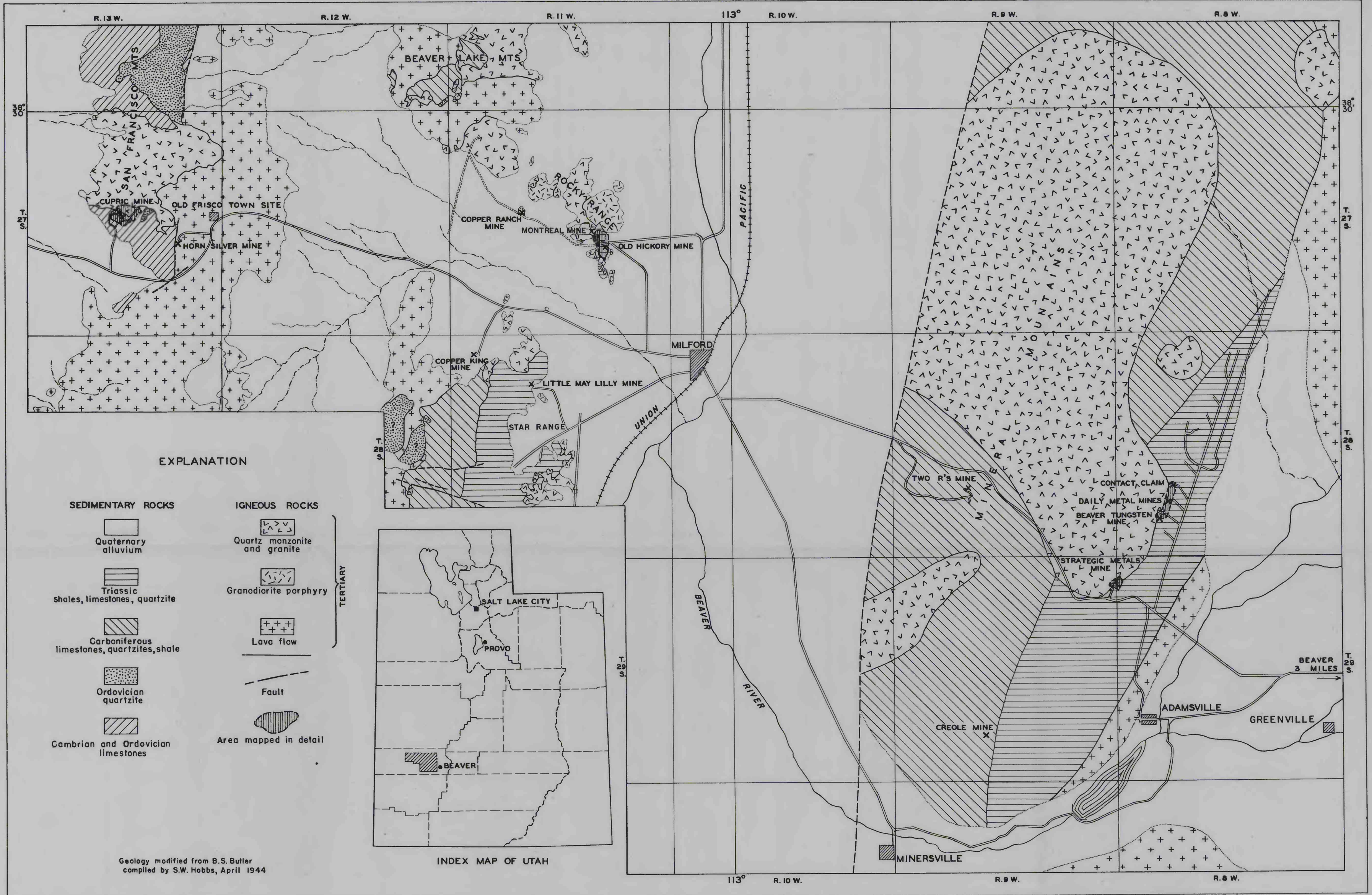
MAP SHOWING LOCATION AND GEOLOGIC SETTING OF THE TUNGSTEN DEPOSITS OF BEAVER COUNTY, UTAH
