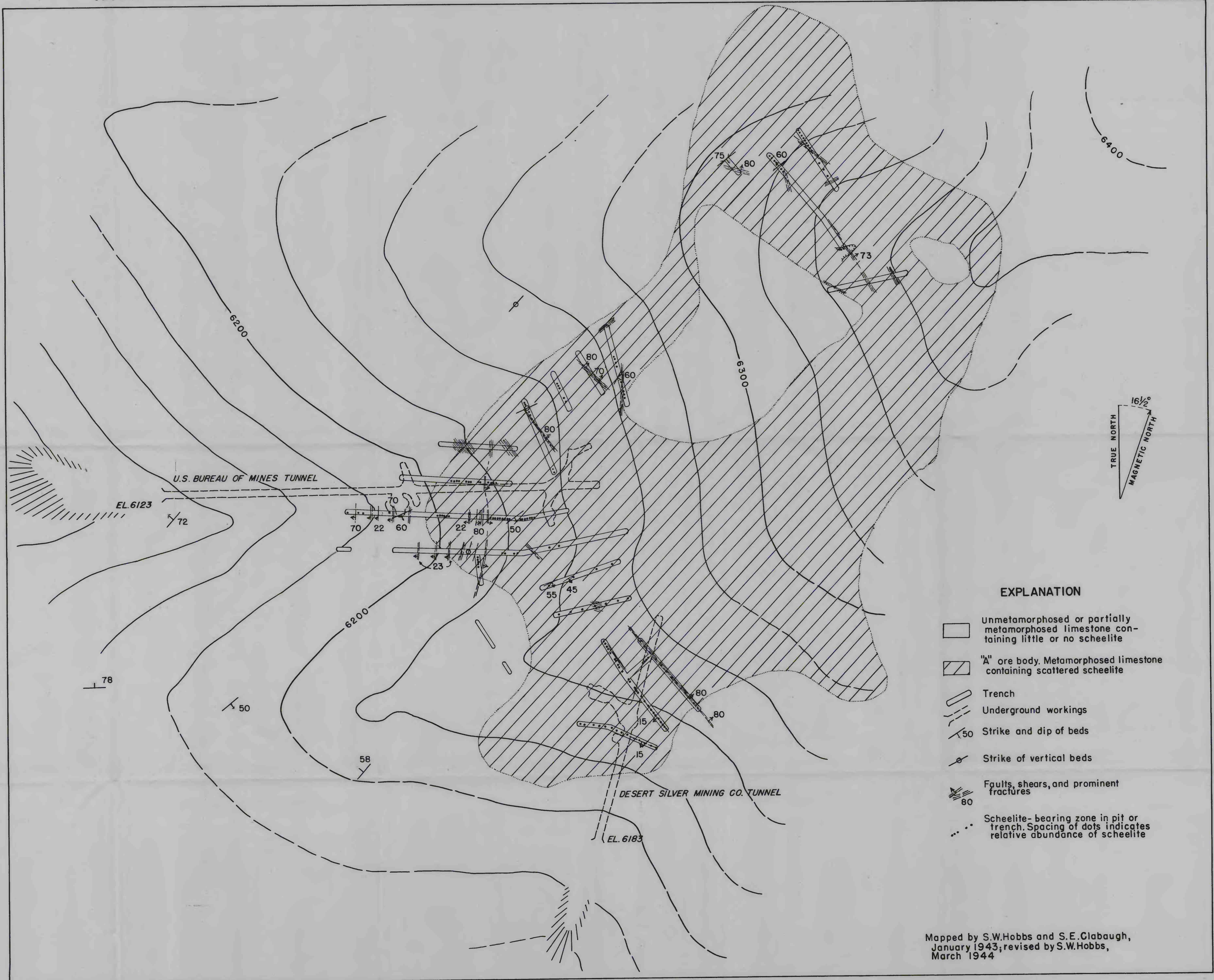
GEOLOGIC MAP OF THE "A" ORE BODY, CUPRIC TUNGSTEN DEPOSIT, BEAVER COUNTY, UTAH
