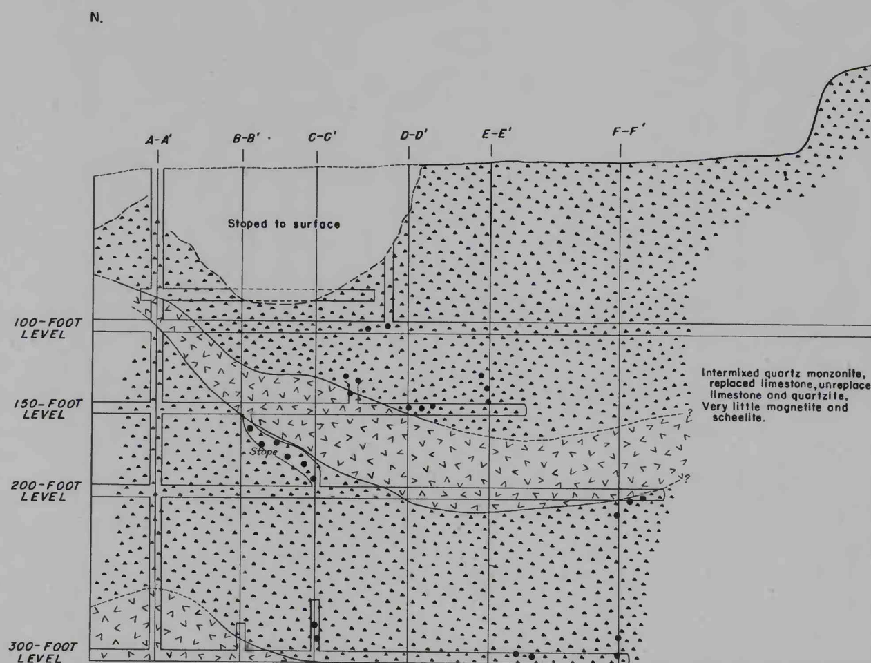
GENERALIZED LONGITUDINAL PROJECTION OF MAGNETITE ORE BODIES
