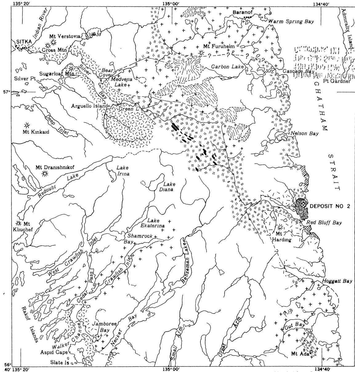
GEOLOGIC RECONNAISSANCE MAP OF CENTRAL BARANOF ISLAND, SOUTHEASTERN ALASKA.
