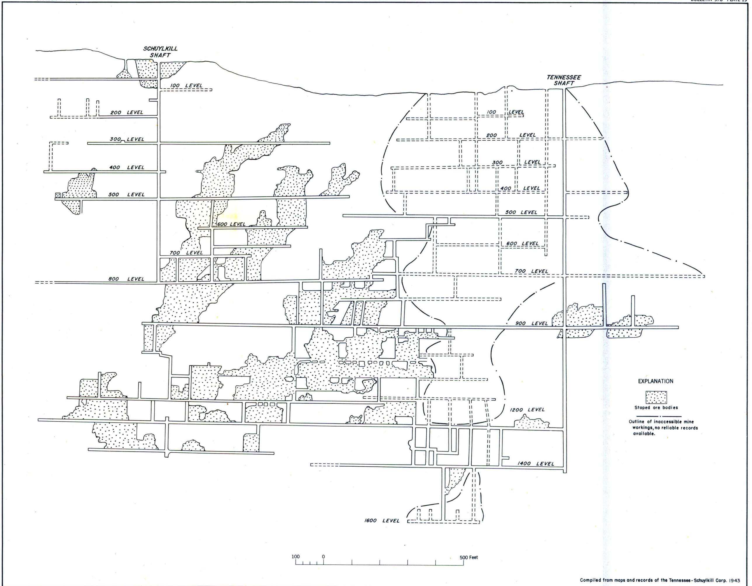
LONGITUDINAL VERTICAL SECTION OF TENNESSEE-SCHUYLKILL MINE, WALLAPAI DISTRICT, ARIZONA, THROUGH TENNESSEE AND SCHUYLKILL SHAFTS. WITH PROJECTION OF MINE WORKINGS AND STOPED ORE BODIES
