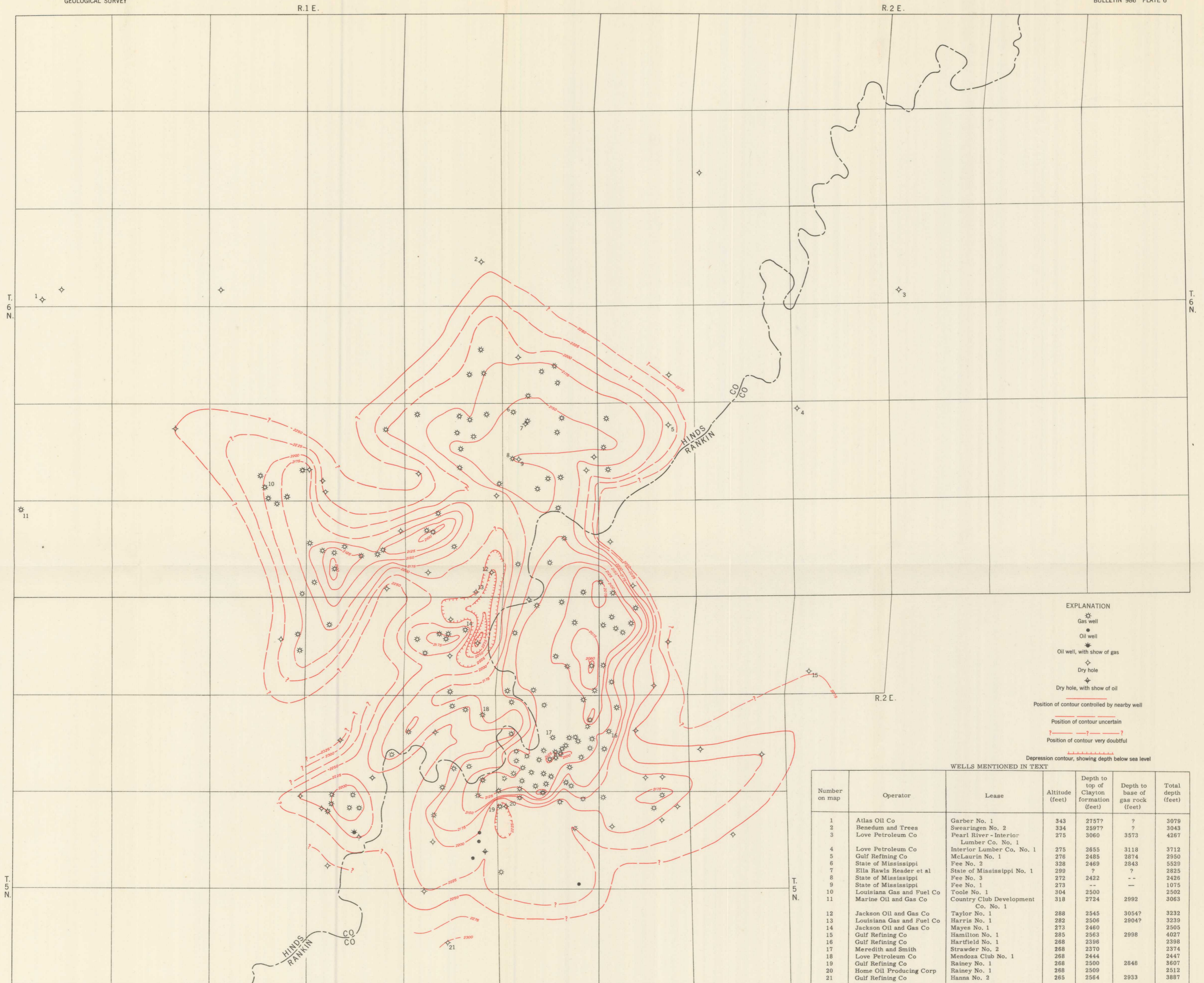
STRUCTURE CONTOUR MAP OF THE TOP OF THE CLAYTON FORMATION IN THE JACKSON GAS FIELD, MISSISSIPPI
