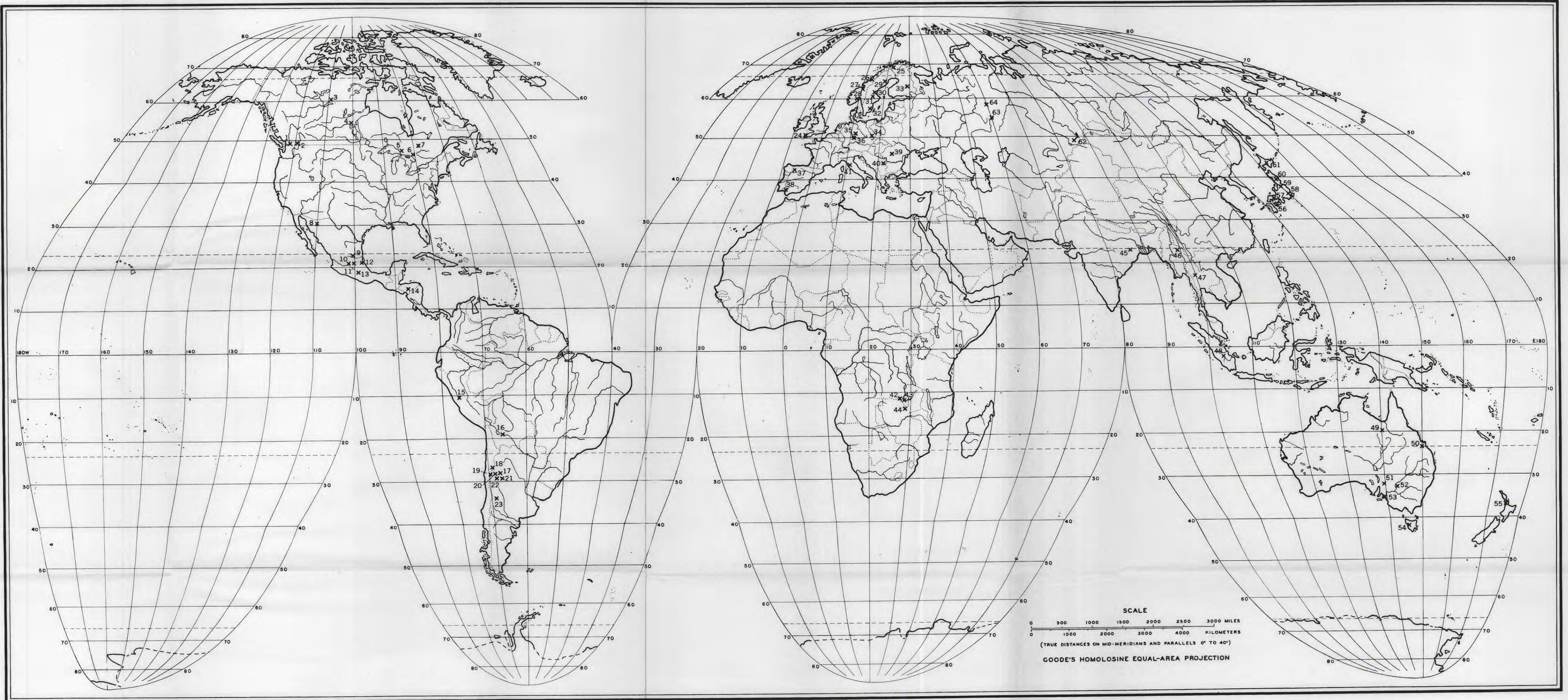
MAP SHOWING SELENIUM-BEARING ORE DEPOSITS OF THE WORLD, EXCEPTING THE UNITED STATES
