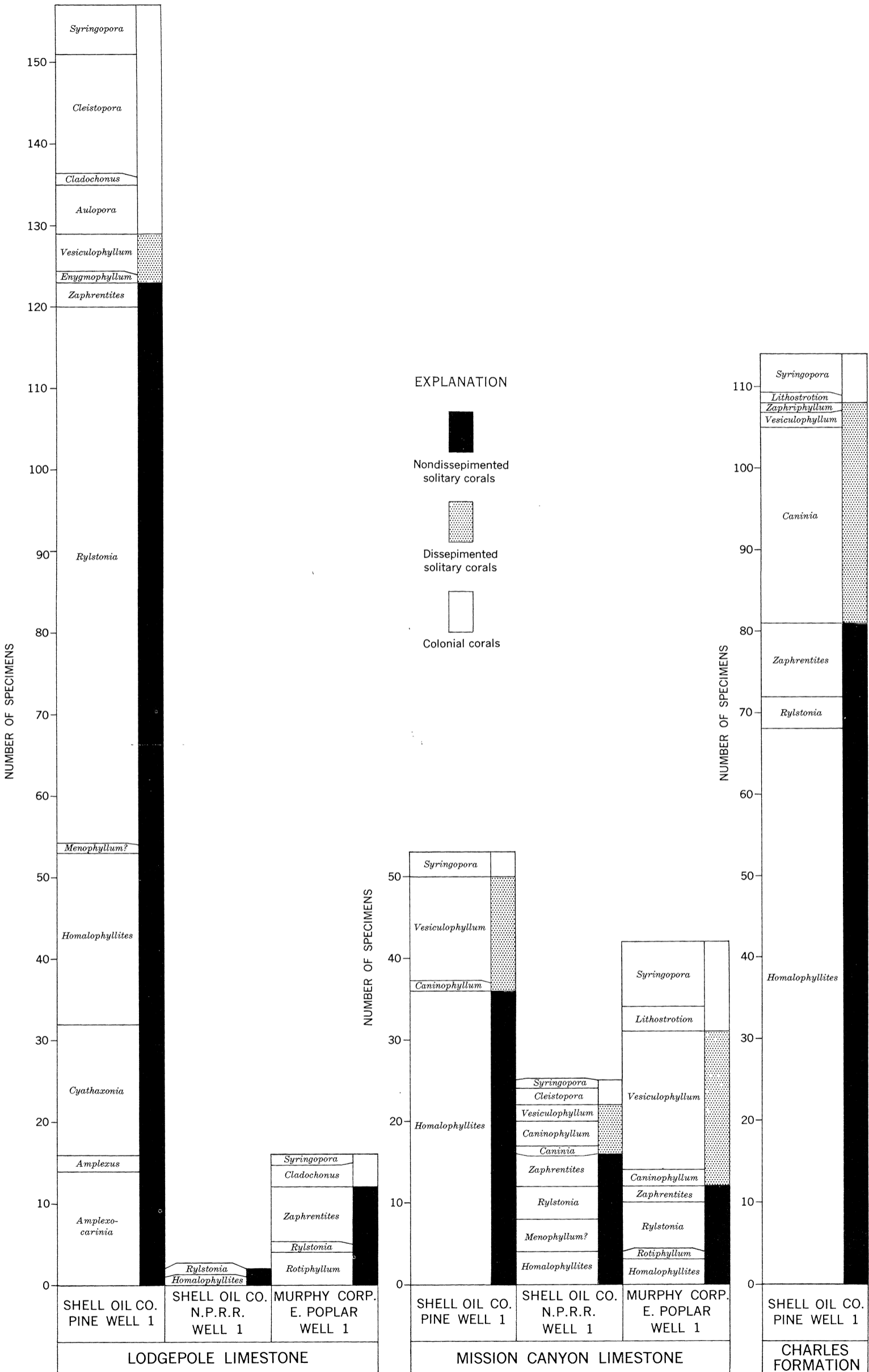
FREQUENCY DISTRIBUTION OF SPECIMENS OF CORAL GENERA IN FORMATIONS OF THE MADISON GROUP
