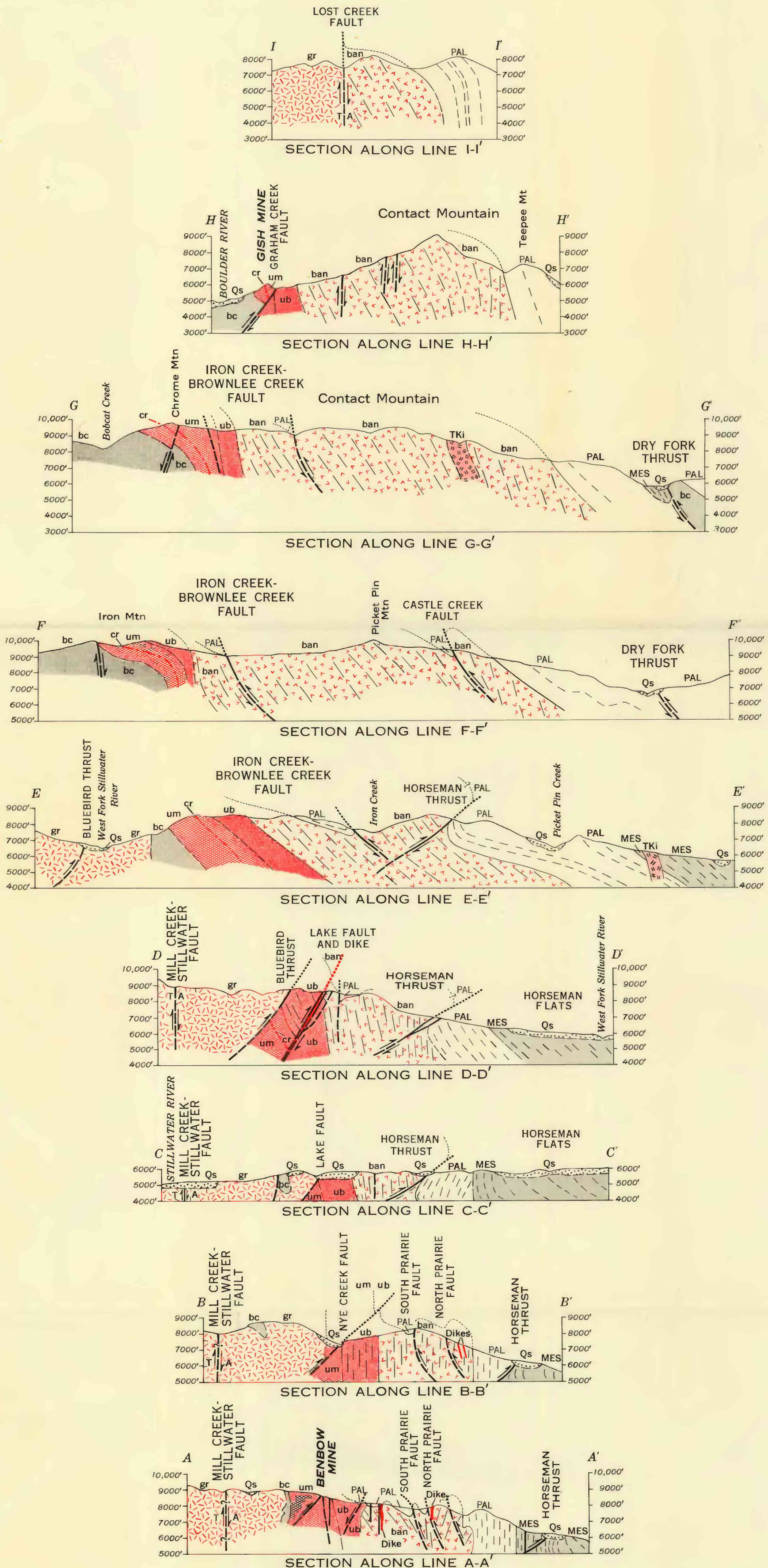
CROSS SECTIONS OF THE STILLWATER COMPLEX, MONTANA
