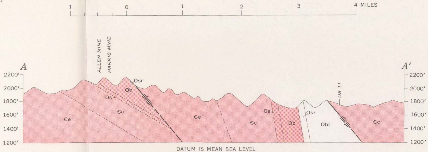
GEOLOGIC MAP AND SECTION, SPOTTSWOOD DISTRICT, VIRGINIA
