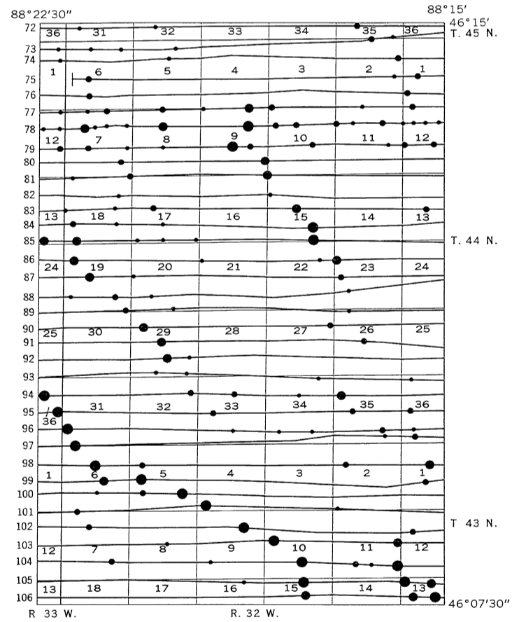
LOCATION OF FLIGHT TRAVERSES AND CRESTS OF AEROMAGNETIC ANOMALIES
