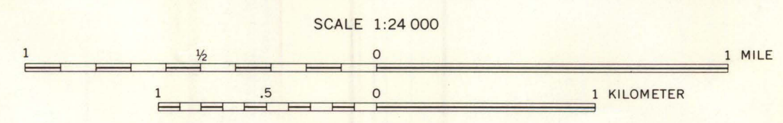
STRUCTURE SECTIONS ACROSS THE TIERRA REDONDA MOUNTAIN AND BRADLEY QUADRANGLES MONTEREY AND SAN LUIS OBISPO COUNTIES, CALIFORNIA
