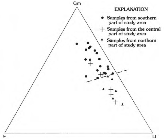
Figure 6. Ternary diagram showing relative amounts of monocrystalline quartz (Qm), total feldspar (F), and total rock fragments (Lt) in sandstones of the Lance Formation, Powder River Basin and Bighorn Basin.
