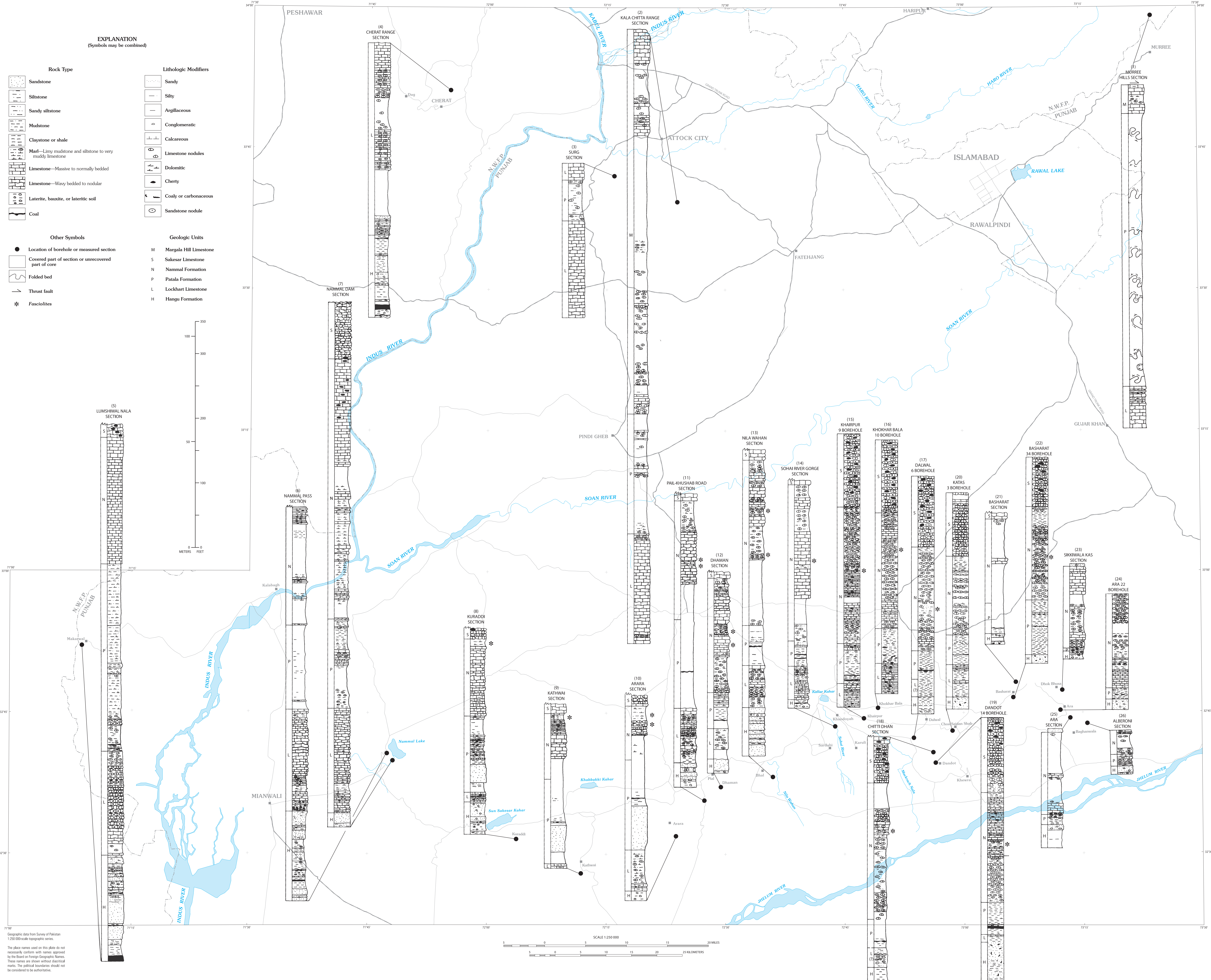
LOCATION AND GRAPHIC DISPLAY OF COLUMNAR SECTIONS FROM THE AREA SURROUNDING THE POTWAR PLATEAU, NORTHERN PAKISTAN
