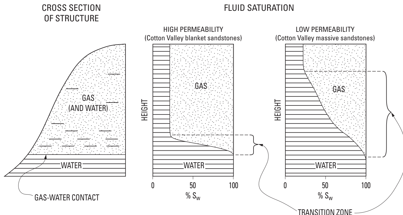
Figure 16. Schematic diagram of gas-water transition zones in high- and low-permeability reservoirs. Modified from Levorsen (1967).
