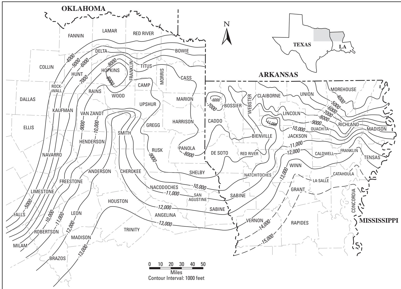
Figure 4. Generalized structure contours on top of Cotton Valley Group sandstone across northeastern Texas and northern Louisiana, modified from Finley (1984). Cotton Valley sandstone has been designated as “tight-gas sandstone” in all counties shown on this map with exception of 15 gas fields in northern Louisiana (fig. 8).
