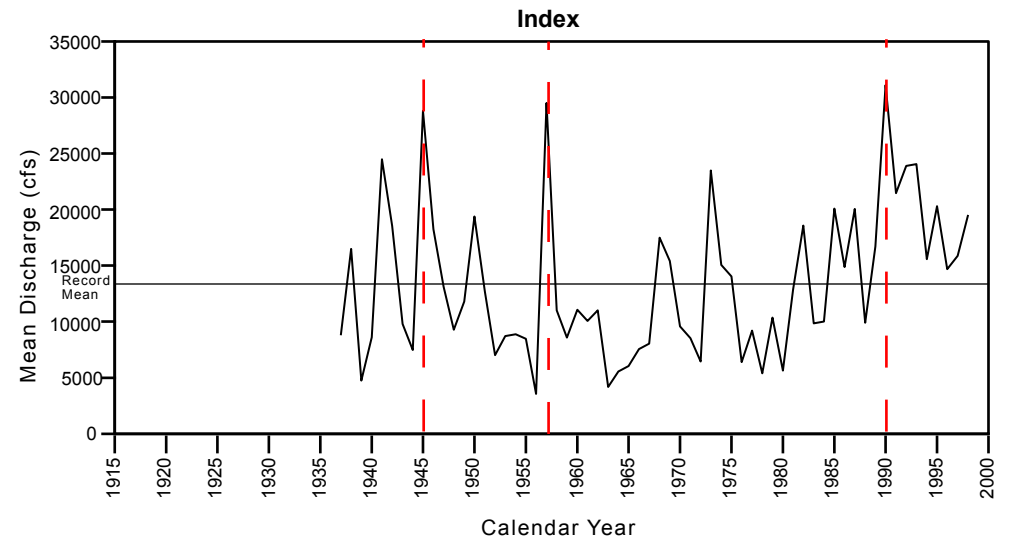
Figure 9. Red River gaging station locations and discharge records. Comparisons of selected gaging station records indicate that mean annual discharge has not been significantly modified by manmade structures. The discharge record for the Arkansas River is repeated from figure 8 for comparison; it shows that the records of the Arkansas River and Red River are similar. Dashed vertical lines track similarities between the records; the horizontal line in each record represents the mean discharge for the entire record. cfs, cubic feet per second.
