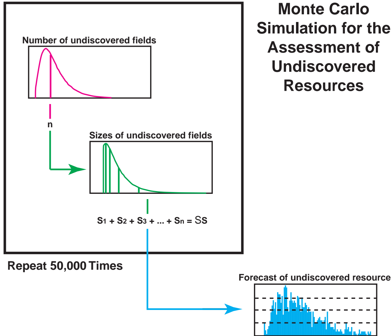
Figure MC-1. Schematic diagram of data model used for Monte Carlo simulation for the assessment of undiscovered resources, used by the programs EMCEE and Emc2 (described in text).
