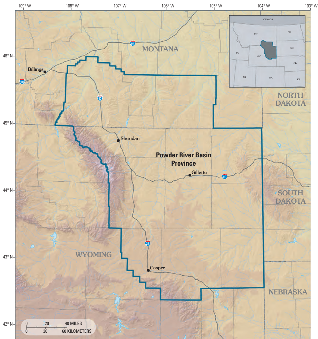
Figure 1. Map showing boundary of Powder River Basin Province in Wyoming and Montana. Province boundary is shown as heavy blue line.
