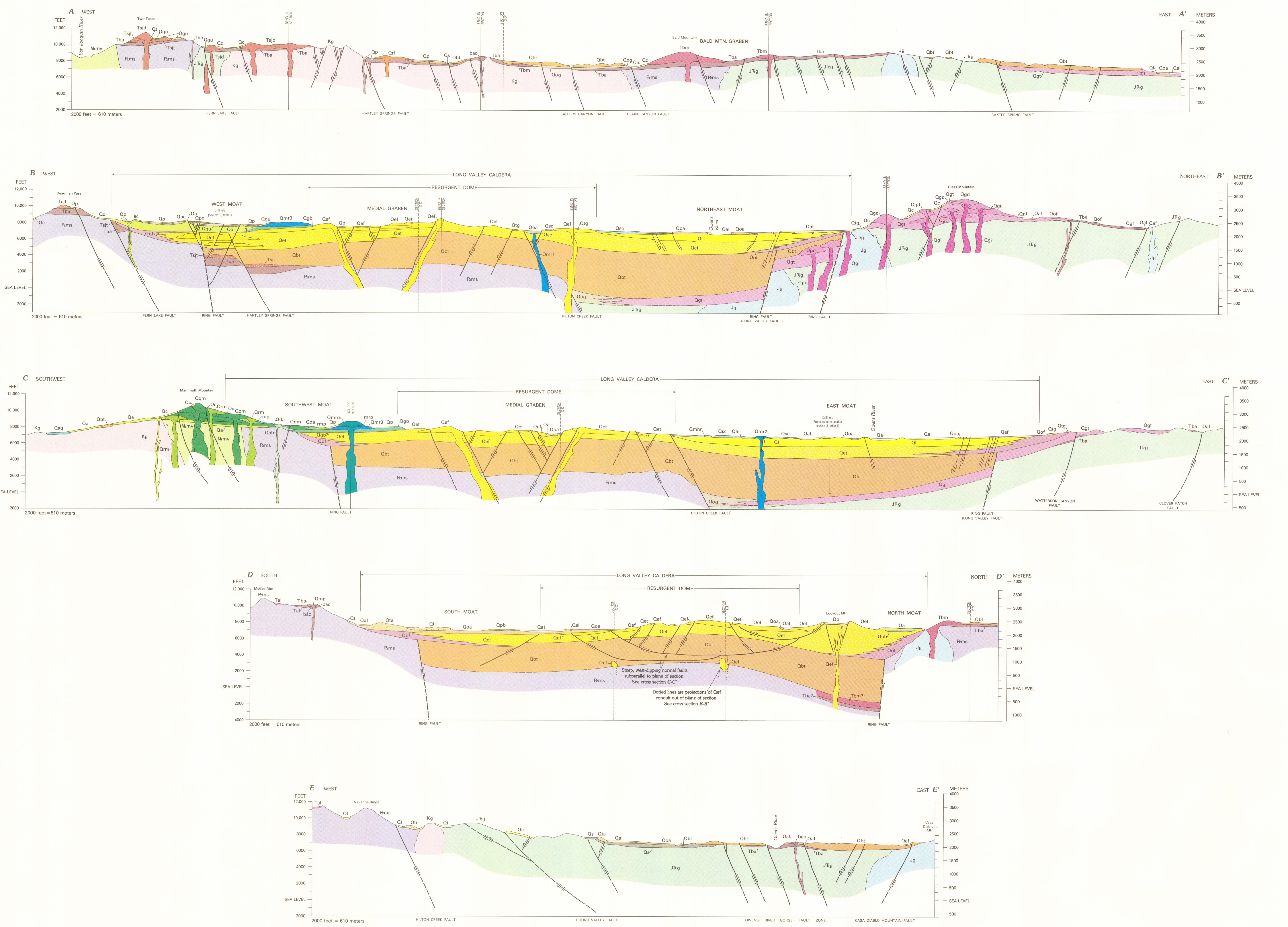
CROSS SECTIONS
