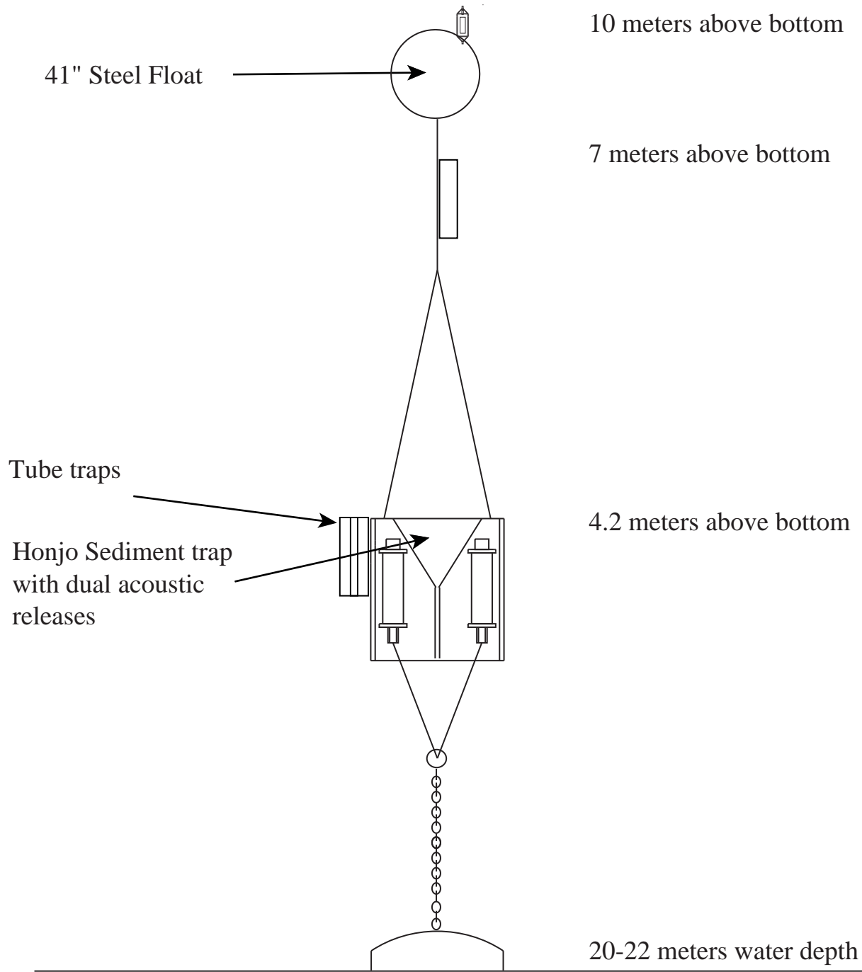
Figure 9B. Schematic of the subsurface mooring deployed at the long-term western Massachusetts Bay Site B from 1997 to 2002. The subsurface mooring supported the time-series sediment trap at 4.2 m above bottom (mab), tube traps at 4.2 and 7 mab, and a MicroCAT at 10 mab. Water depth ranged from 20 to 22 m.
