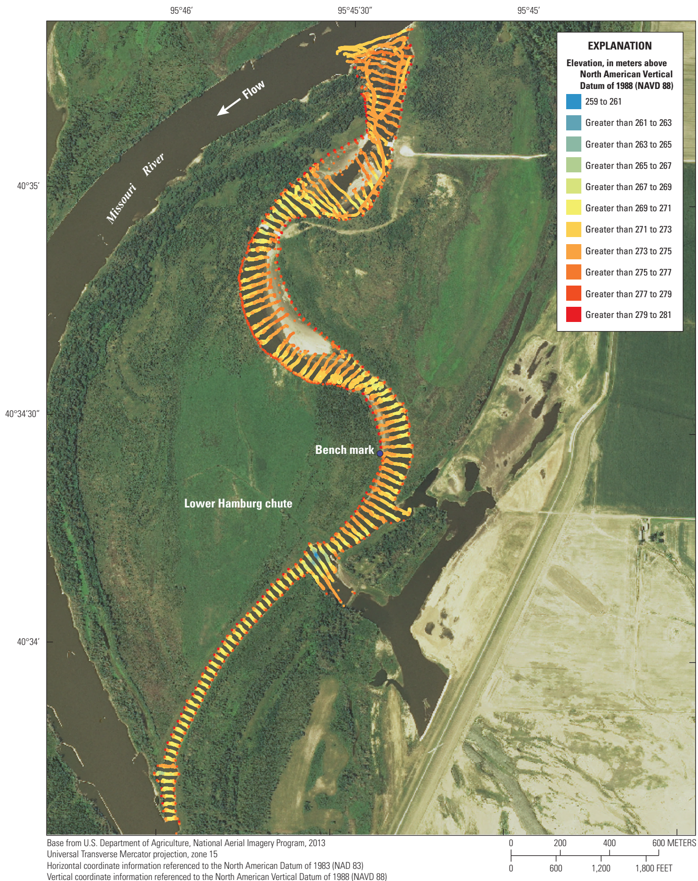
Figure 10. Hydrographic survey data for Lower Hamburg chute near Hamburg, Iowa, 2011–13.
