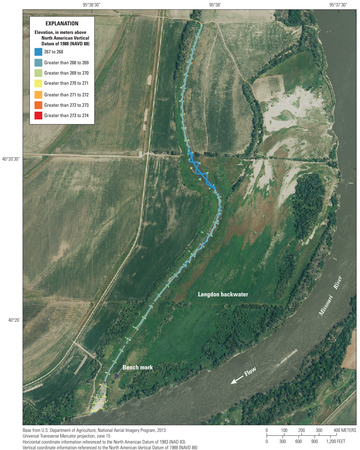
Figure 12. Hydrographic survey data for Langdon backwater near Nemaha, Nebraska, 2011–13.
