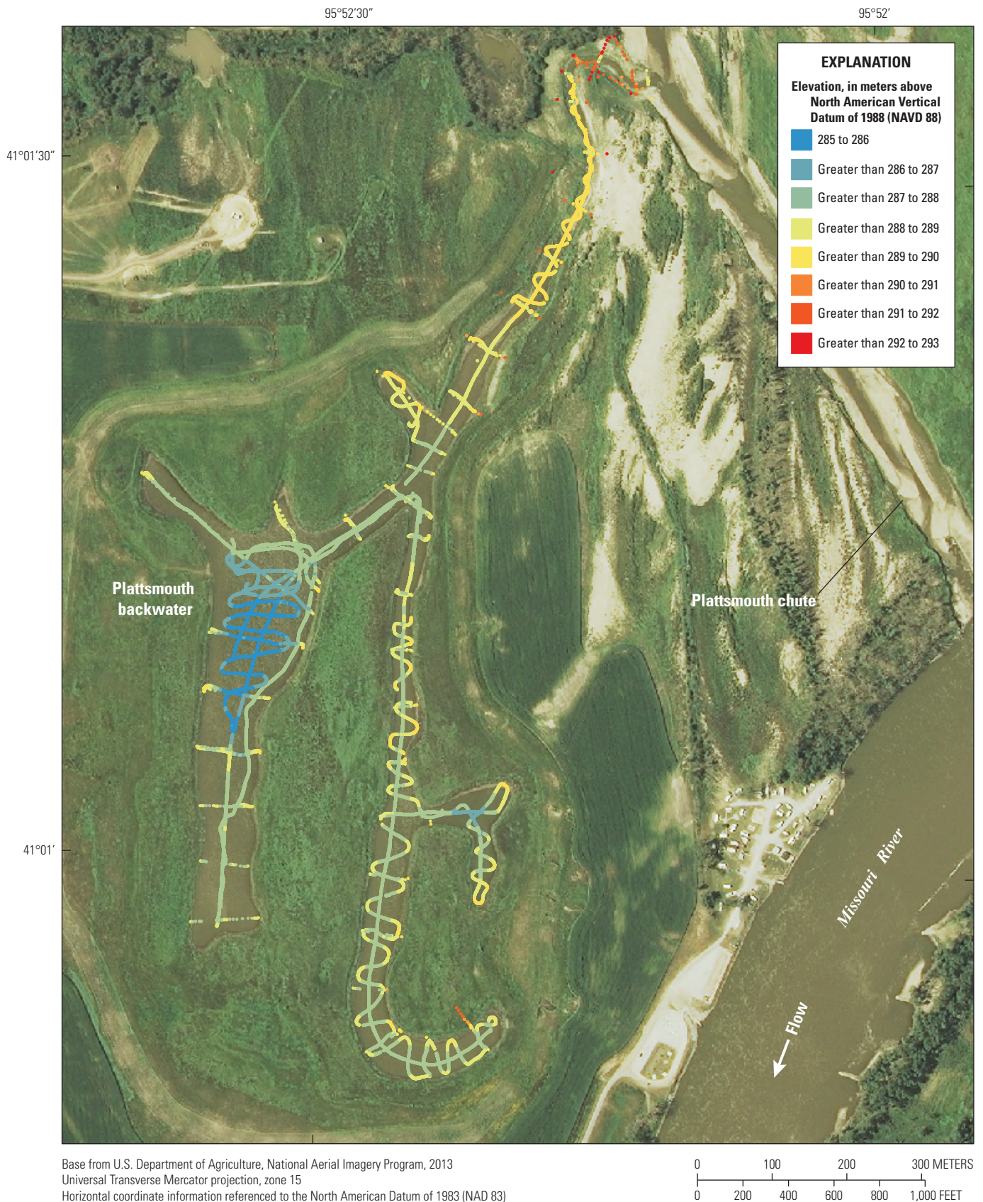
Figure 7. Hydrographic survey data for Plattsmouth backwater near Plattsmouth, Nebraska, 2011–13.
