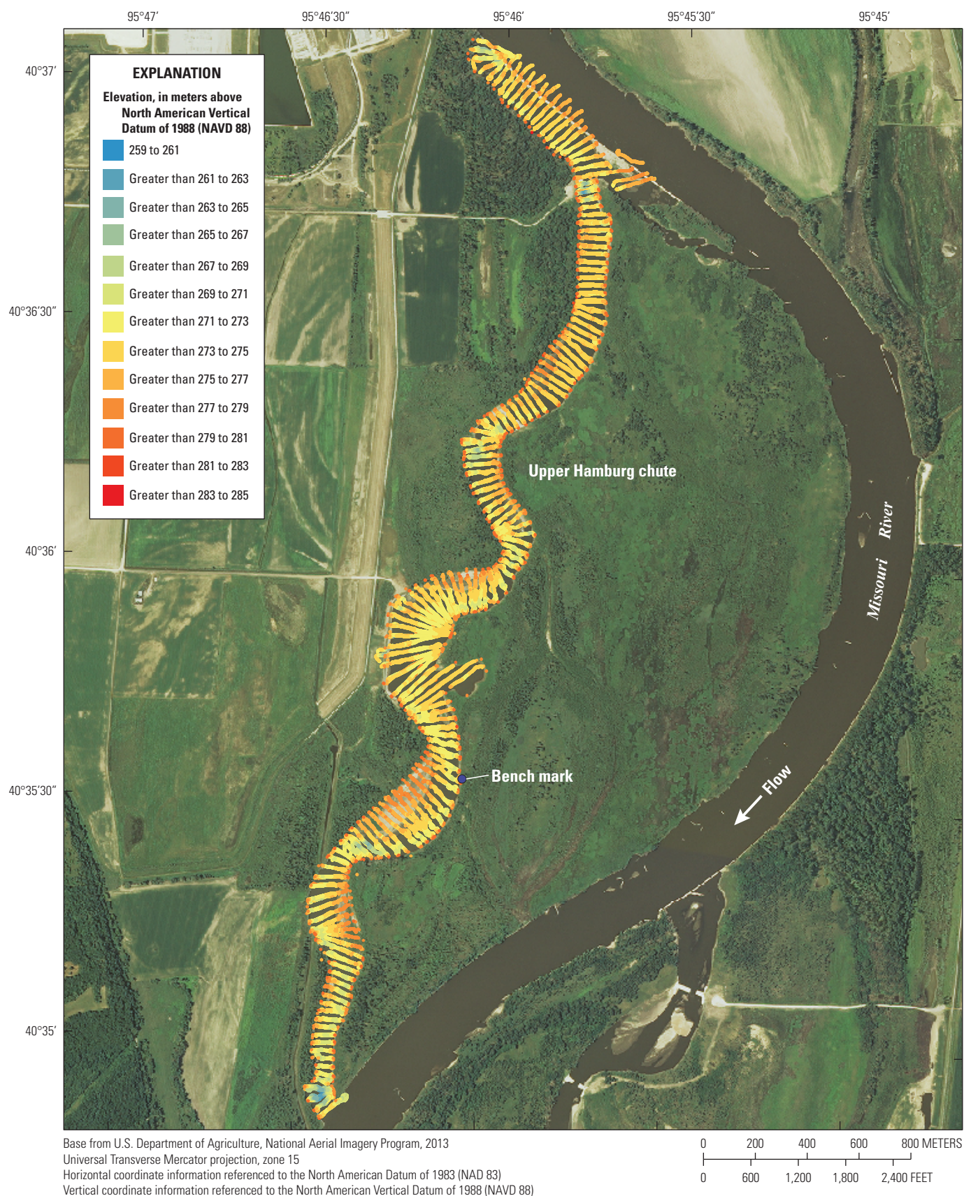
Figure 9. Hydrographic survey data for Upper Hamburg chute near Nebraska City, Nebraska, 2011–13.
