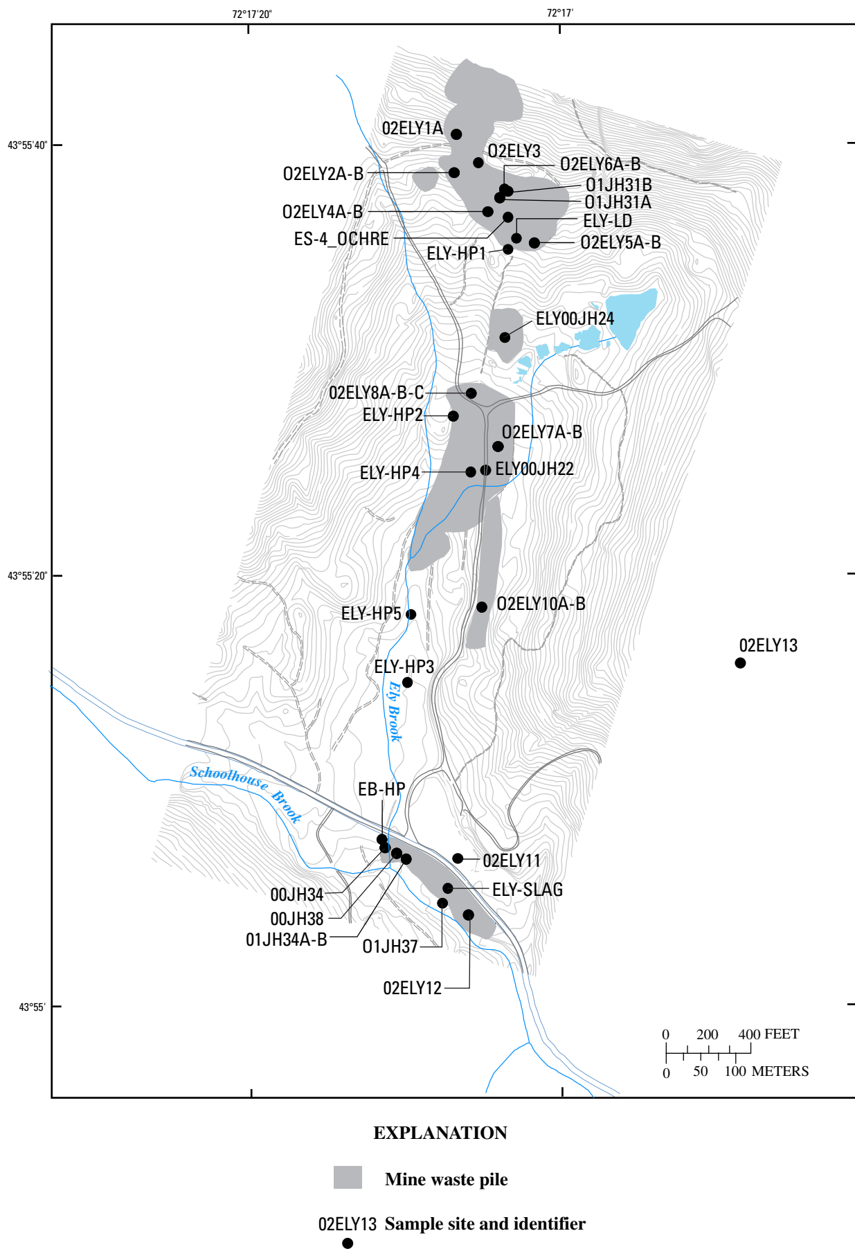
Figure 3. Location of soil samples collected in and around the piles of mine waste at the Ely Copper Mine Superfund site in Vershire, Vermont. The sample from location 02ELY13 was collected near the end of a smoke flue which previously had been connected to a smelter.
