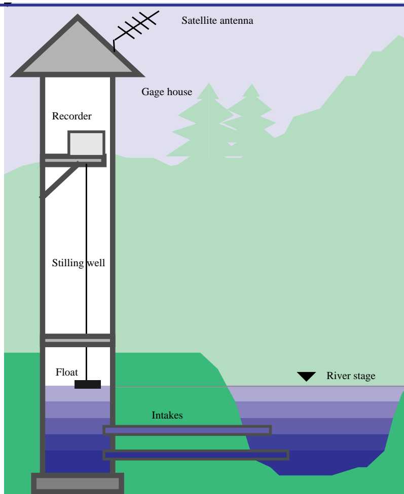
Figure 1. Sketch of a U.S. Geological Survey streamflow-gaging station.
