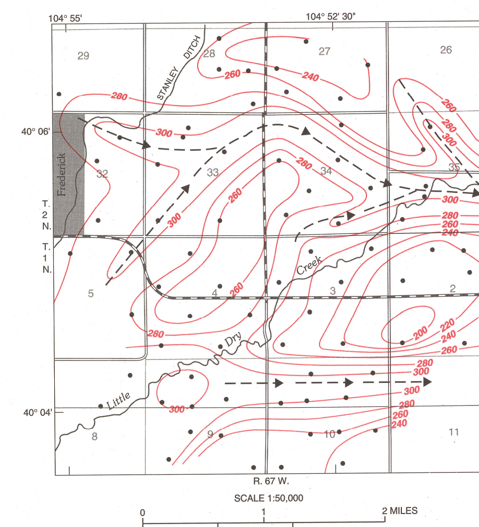
FIGURE 5 Thickness of Laramie-Fox Hills aquifer in area east of Frederick
