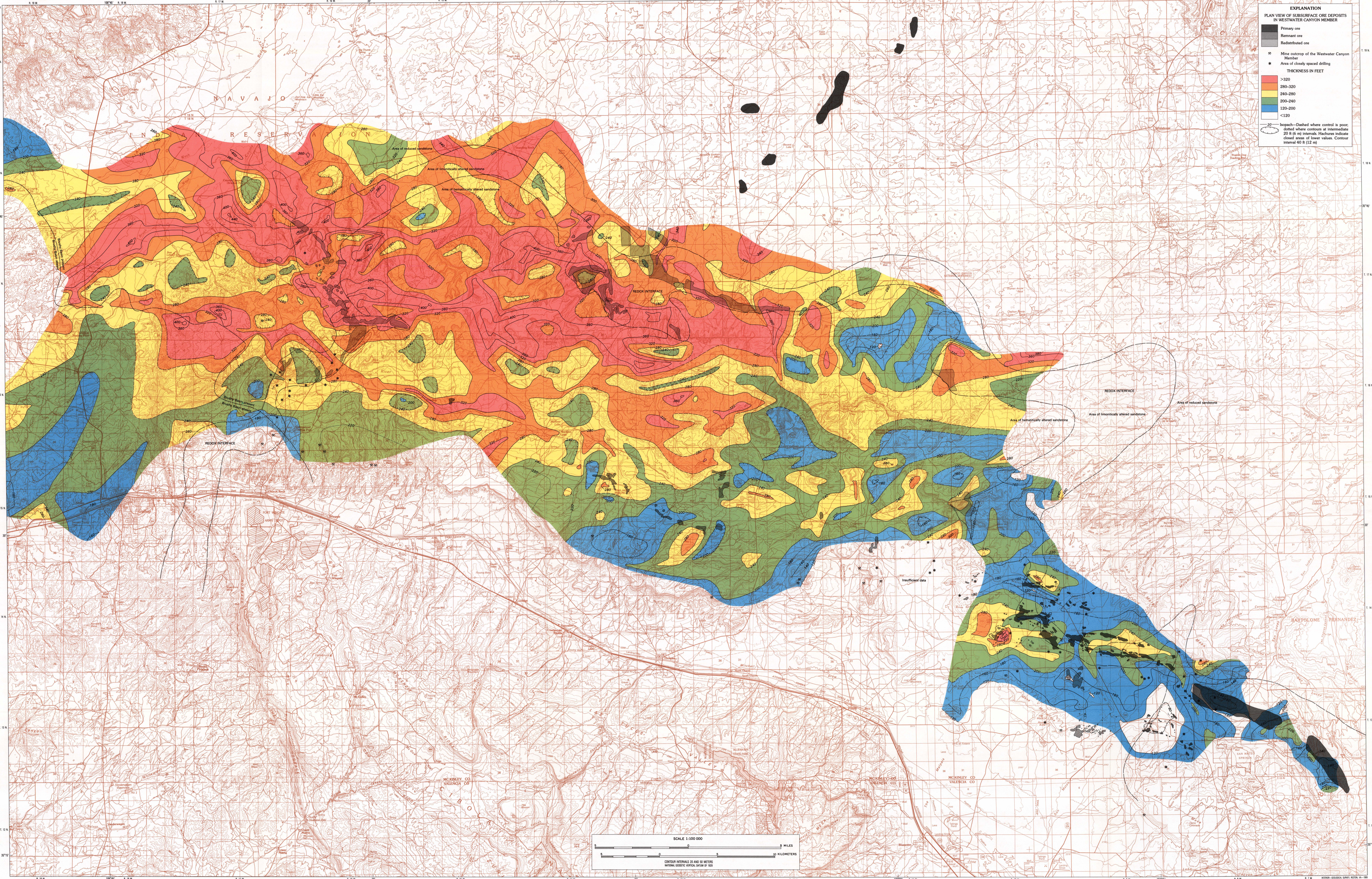
Isopach map of the Westwater Canyon Member of the Morrison Formation ISOPACH MAPS OF THE WESTWATER CANYON AND BRUSHY BASIN MEMBERS OF THE MORRISON FORMATION, SHOWING STRUCTURAL CONTROL OF SEDIMENTATION PATTERNS AND URANIUM DEPOSITS, SAN JUAN BASIN, NEW MEXICO
