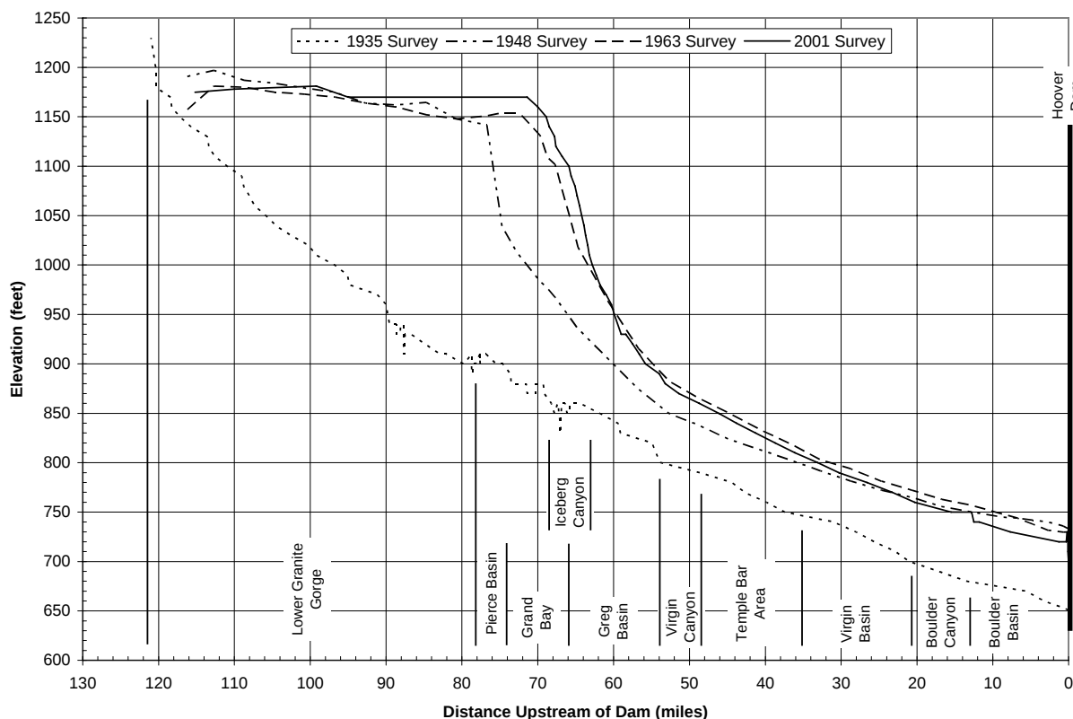
Figure 4 1935, 1948, 1963, and 2001 Colorado River profiles through Lake Mead
