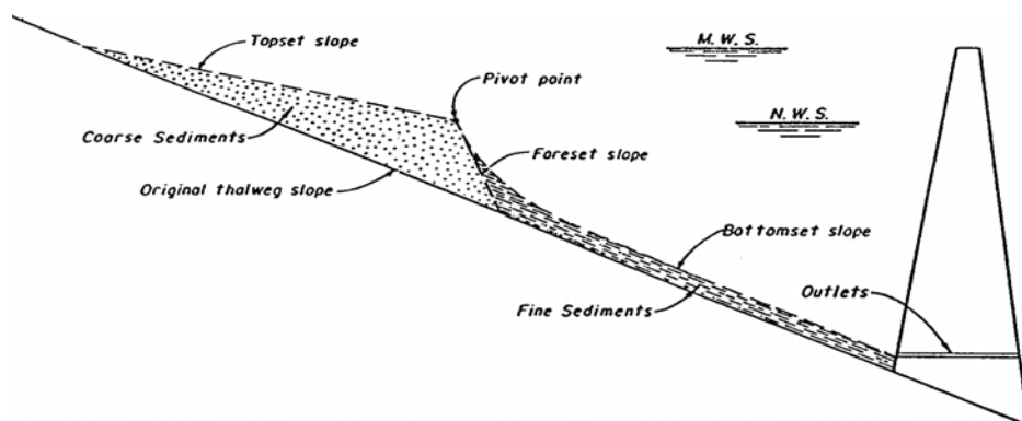
Figure 1 Profile of reservoir delta formation
