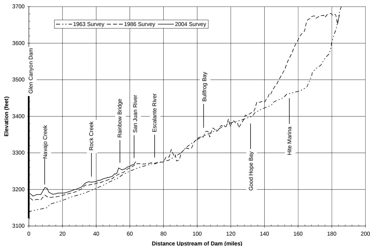
Figure 7 1963, 1986, and 2004 Colorado River Profiles through Lake Powell
