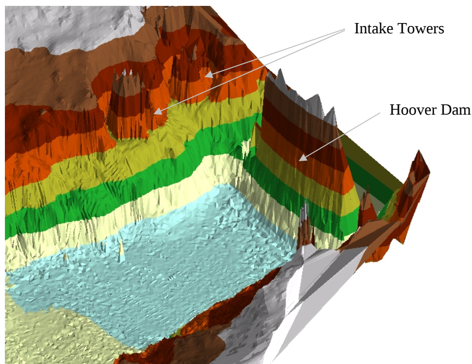
Figure 3 Multibeam image of Hoover Dam and intake towers
