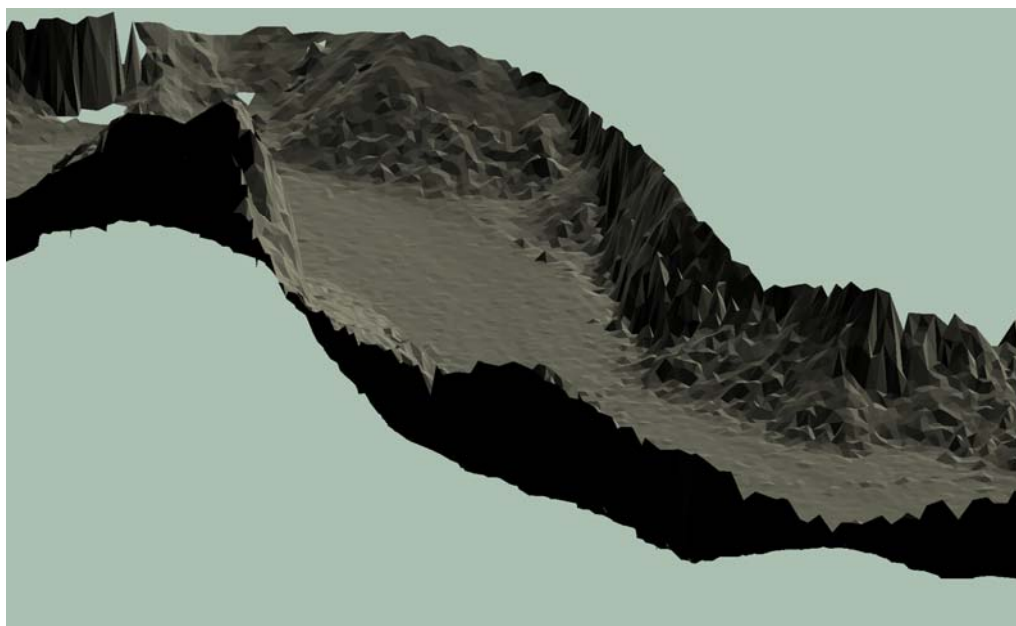
Figure 5 Navajo Canyon TIN generated from multibeam data only
