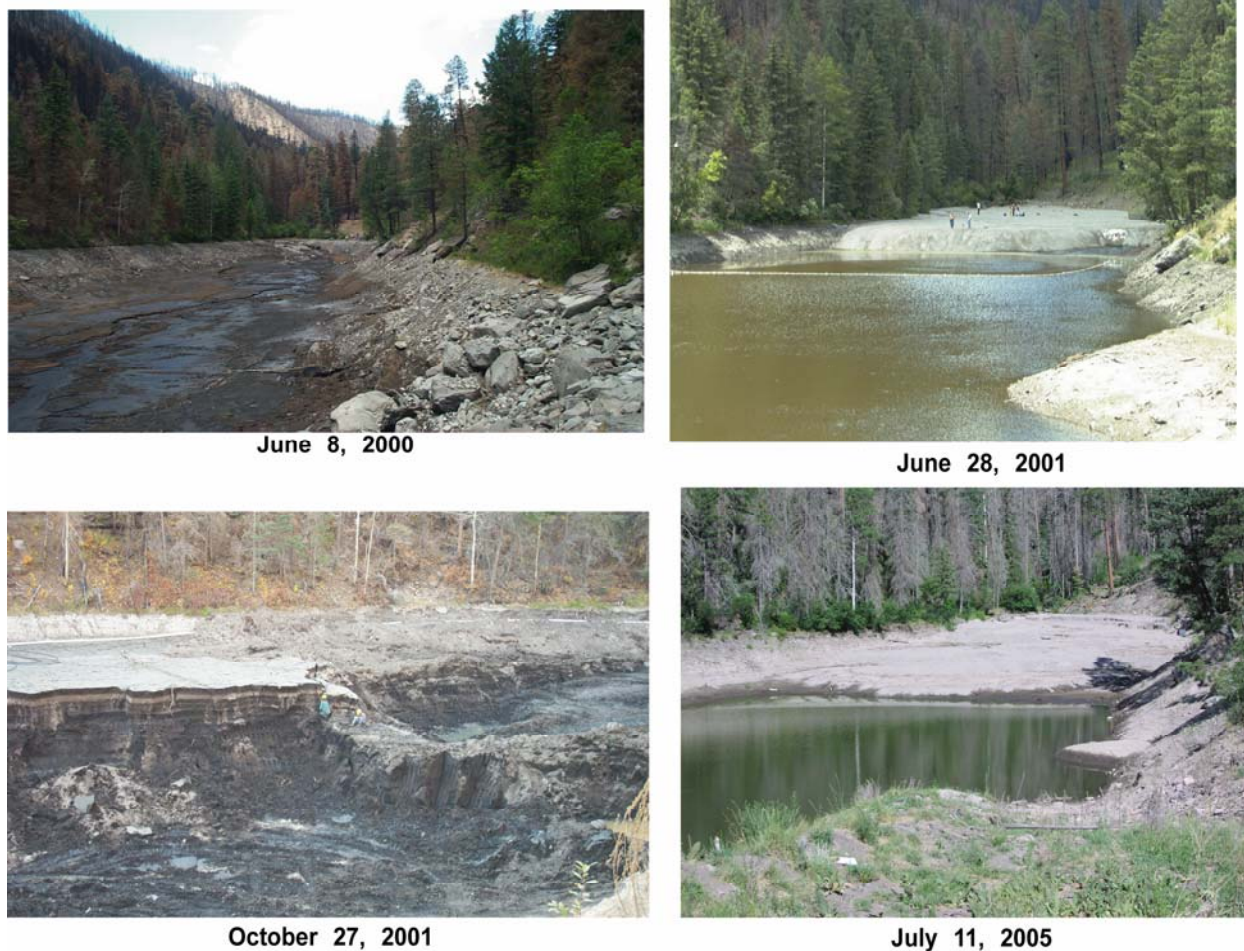
Figure 3 Photographs of the Los Alamos Reservoir: June 8, 2000, drained, after a single post-fire flood: June 28, 2001, showing a large coarse-grained delta that was formed during snowmelt runoff in spring 2001: October 27, 2001, partially excavated, showing fine-grained post-fire sediment deposits, people in center are describing stratigraphic section shown in Figure 4: July 11, 2005, showing delta formed during snowmelt runoff in spring 2005.
