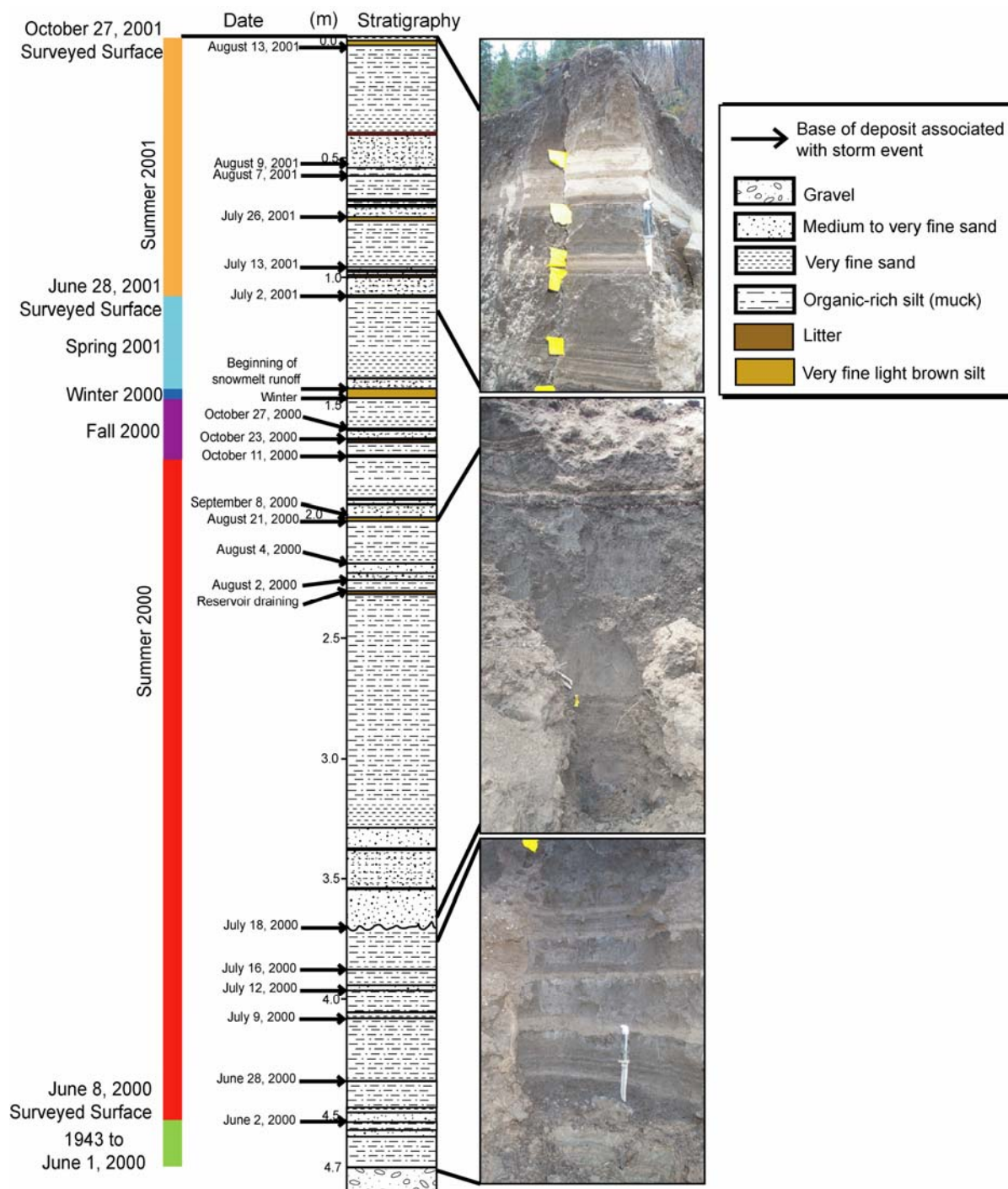
Figure 4 Stratigraphy exposed in excavation at the reservoir on October 27, 2001. Surveyed elevations, precipitation data, and field observations allowed correlation of individual layers to specific storms. More than 3 m of sediment were deposited during the first year following the fire, close to half of this following the July 18, 2000 storm, compared with ~0.2 m in the prior 57 years.
