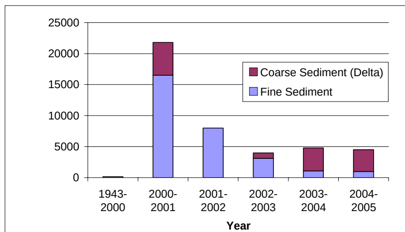
Figure 5 Plot of annual sedimentation in the reservoir, distinguishing coarse-grained sediment in the delta that predominantly reflects snowmelt runoff and fine-grained sediment that predominantly reflects suspended transport in summer floods. Note the overall annual decrease in the amount of fine sediments, and the relative increase in the percentage of coarse-grained to fine-grained sediments. 1943-2000 value is a 57-year average.
