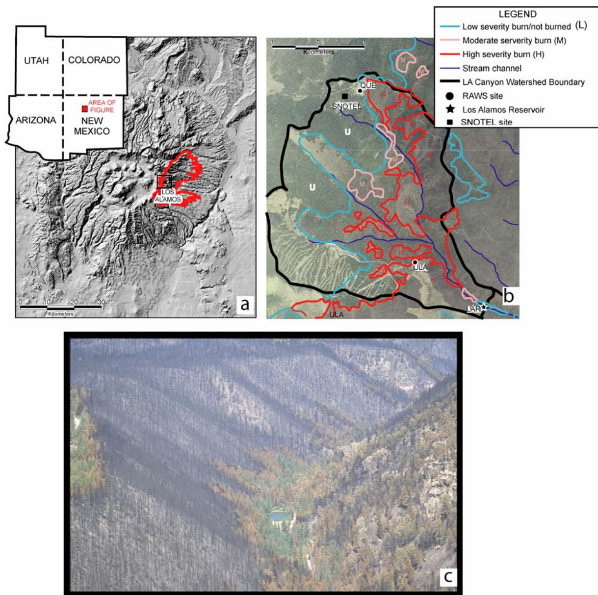
Figure 1 a) Map showing the location of the Cerro Grande fire in north-central New Mexico. Black outline shows area of Figure 1b. b) Aerial photograph showing burn severity in the Los Alamos Reservoir (LAR) watershed; QUE and ULA are RAWS sites; “U” indicates unburned areas; some of the high-severity burn areas have been treated with straw mulch (e.g., southeast of ULA RAWS). c) Oblique-aerial photograph of Los Alamos Canyon and reservoir, looking upstream, shortly after the Cerro Grande fire.
