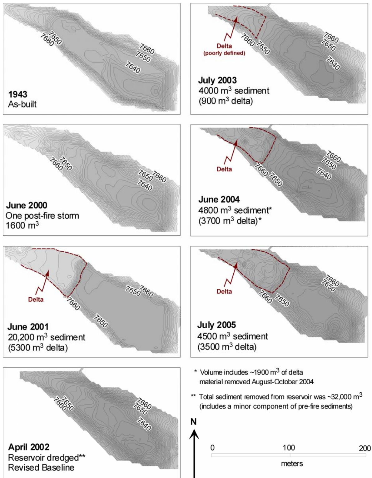
Figure 2 Series of contour maps showing changes in the topography of the reservoir basin based on total station surveys and an as-built survey (1943). Contour interval is 1 foot (0.3 m). Volumes shown reflect amount of sediment deposited between surveys.
