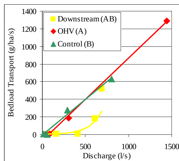
Figure 8 Bed load sediment transport for each reach.
