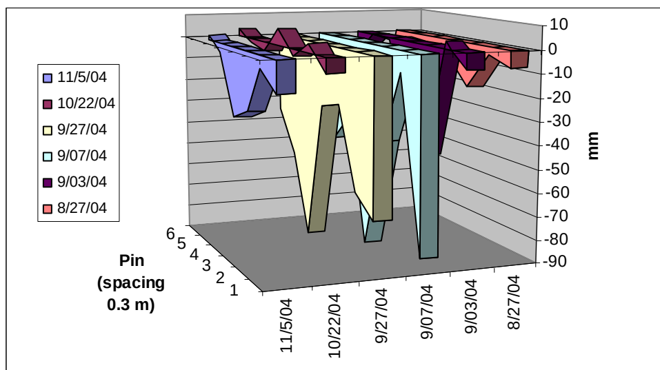
Figure 9 Scour and deposition of the stream bed at OHV Site A. Negative and positive values indicate event scour and deposition on a per event basis. Relative throughput of bed load sediment through the reach can be inferred from the area of each curve. The pre and post stream bed cross section elevations were quite similar following each event (no significant net change in bed elevation). October and November data are inaccurate from debris on pins.
