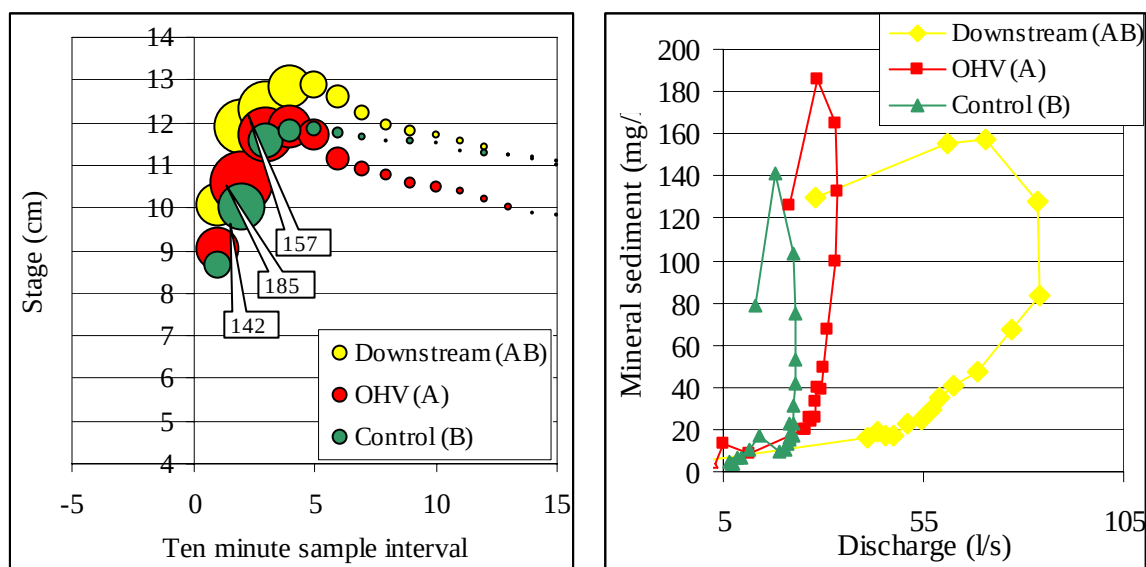
Figure 5a Sedigraph showing concentrations of sediment during a storm event. Bubble size indicates relative concentration and numbers show peak concentrations (mg/l).
