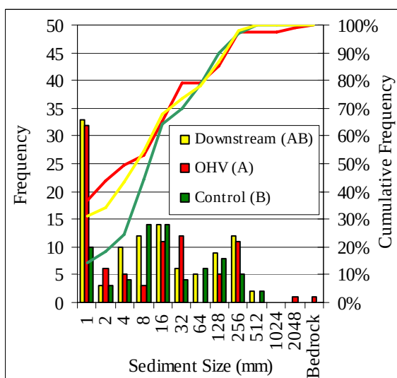
Figure 7 Particle size distributions of stream bed sediments.
