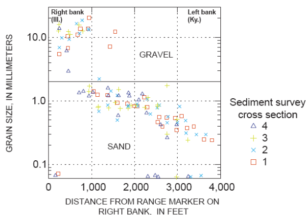
Figure 3 Summary of the bed-material D_{50} for sediment samples collected at four cross sections located around the mussel beds in the Olmsted Locks and Dam study reach near Olmsted, Ill.
