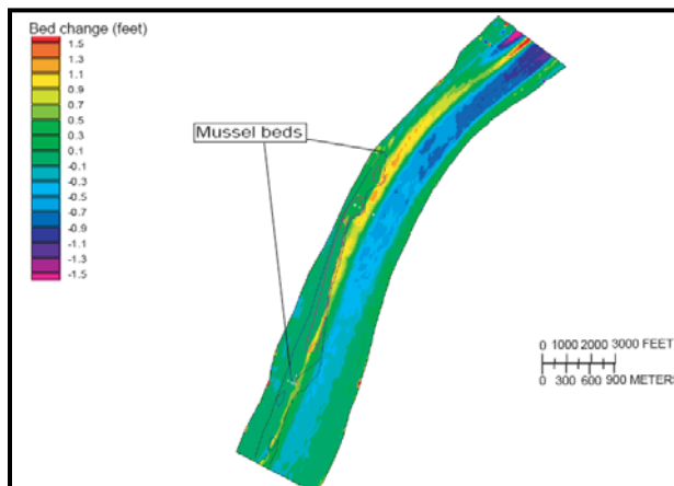
Figure 4 Difference in bed change between baseline and construction simulations after year 6 in the Olmsted Locks and Dam study reach near Olmsted, Illinois.
