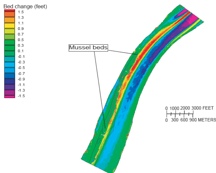
Figure 6 Difference in bed change between baseline and fully operational locks and dam simulation after year 9 in the Olmsted Locks and Dam study reach near Olmsted, Illinois.
