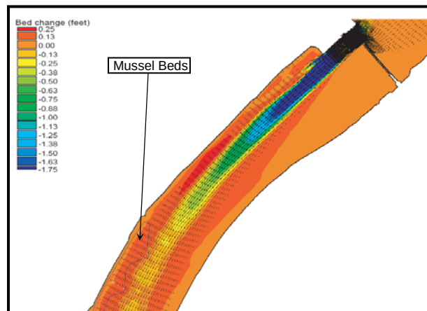
Figure 5. Difference in bed change between baseline and construction simulations after year 5, superimposed with hydraulics for a low-flow model simulation of Olmsted Locks and Dam.
