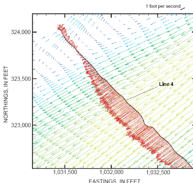
Figure 2 ADCP-measured and simulated low-flow velocity vectors at a cross-section in the Olmsted Locks and Dam study reach near Olmsted, Illinois (red arrows represent field data, multi-colored arrows represent model data)
