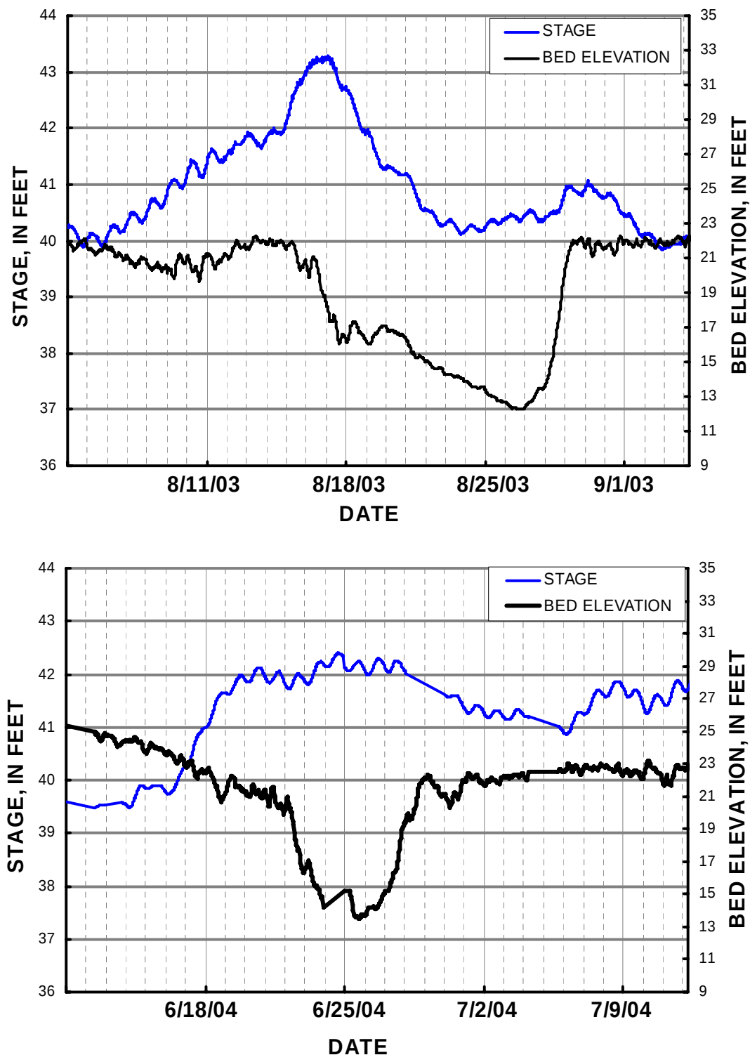
Figure 4 Stage and bed elevation at monitored bridge pier from two scour and fill events on the Knik River near Palmer, Alaska. Stage increases were the result of rainfall (2003, upper plot) and glacial melting from a prolonged period of warm weather (2004, lower plot).
