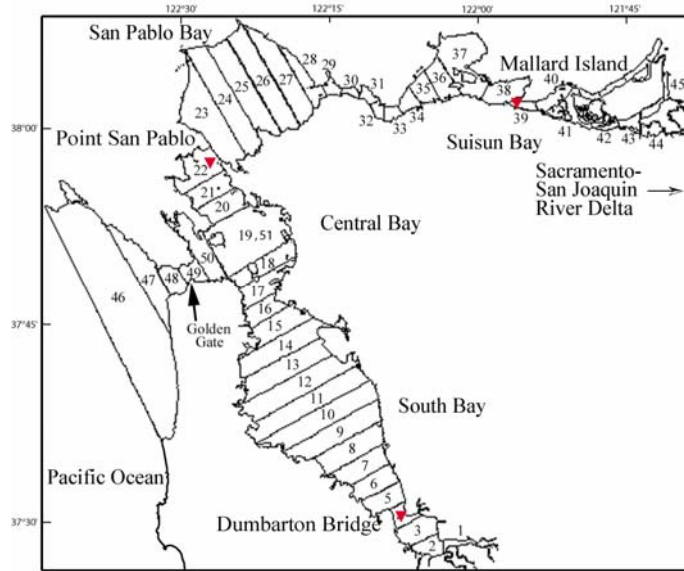
Figure 1 UP model segmentation of the San Francisco Bay (Uncles and Peterson 1995).
