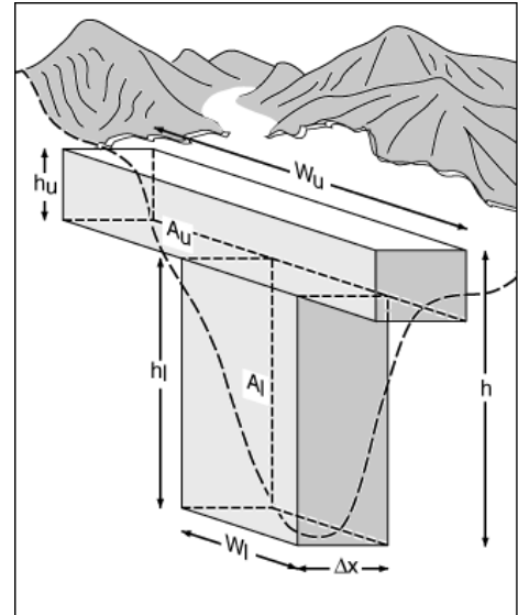
Figure 2 2-layer box composition of the UP box segments (Uncles and Peterson 1995).
