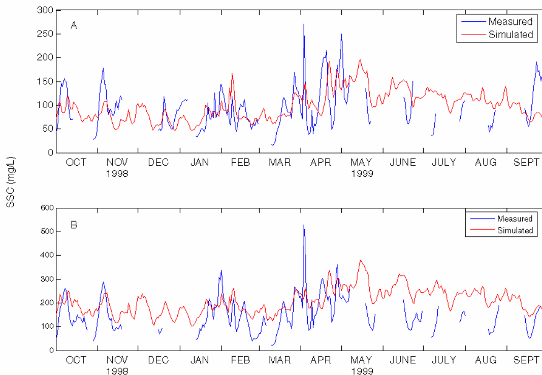
Figure 3 Simulated SSC for water year 1999 at Dumbarton Bridge (A) at mid depth (22 ft below MLLW) and (B) at near bottom (41 ft below MLLW).
