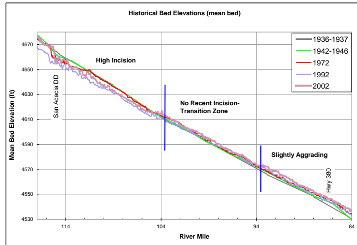
Figure 3 Sample of the Rio Grande bed elevation data available for the Middle Rio Grande; San Acacia Diversion Dam to the U.S. Highway 380 crossing near San Antonio, NM.
