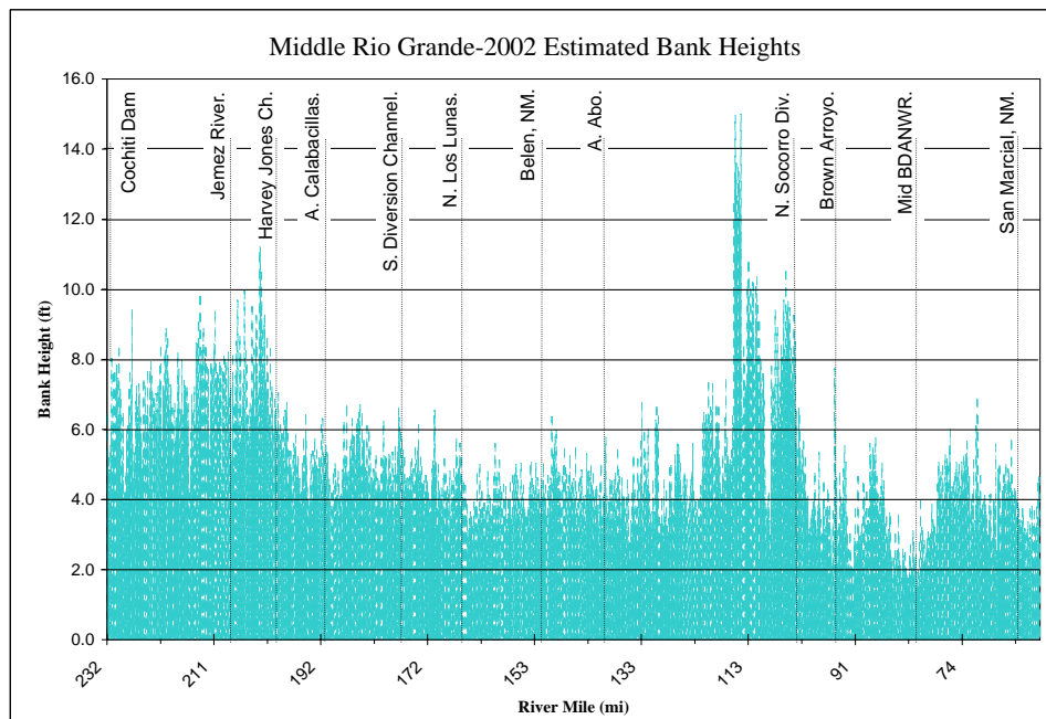
Figure 4 Estimated bank height for the MRG based on cross section data.
