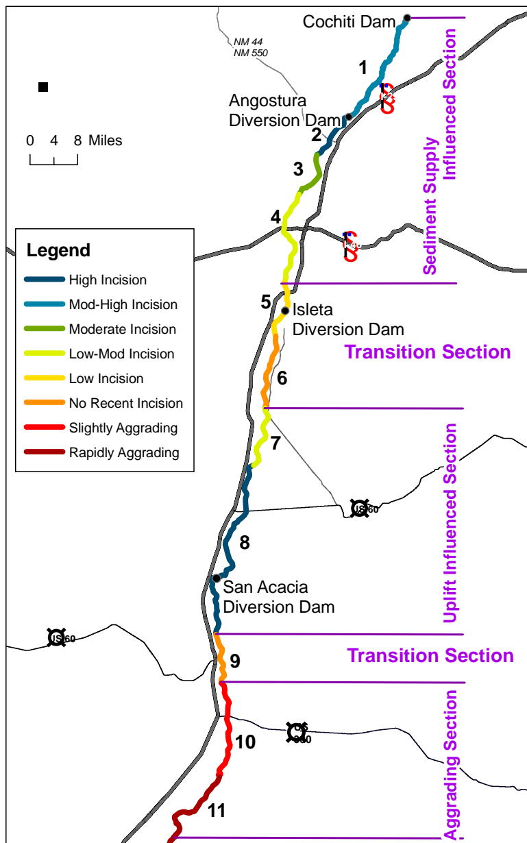
Figure 5 Summary figure showing incision trends from Cochiti Dam to Elephant Butte Reservoir, NM; numbers correspond to reach descriptions in the text. Channel descriptions are as follows: high incision has bank heights >6 ft.; moderate incision has bank heights 3-5 ft.; low incision has bank heights <3 ft.; slightly aggrading channels have <10 ft. of aggradation since 1935, while the rapidly aggrading is >10 ft. of aggradation; combination descriptions (i.e., Mod-High) indicates a mixture of bank heights.
