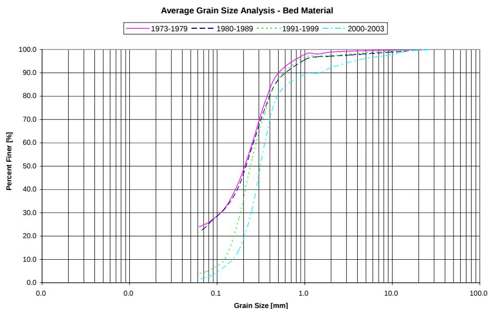
Figure 3 Average Grain Size Analysis for the Bed Material over Time (1973-2003)
