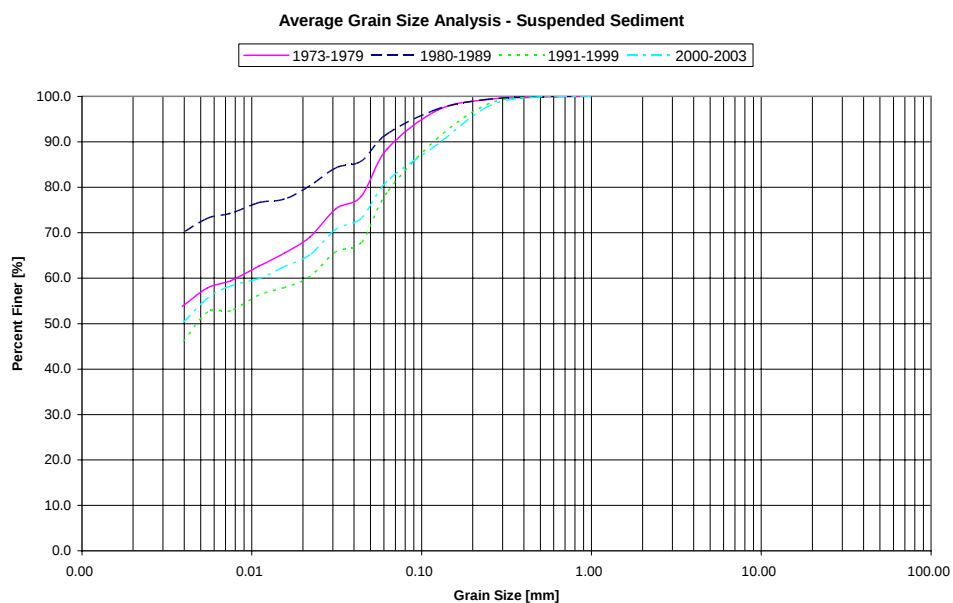
Figure 4 Average Grain Size Analysis for the Suspended Material over Time (1973-2003)
