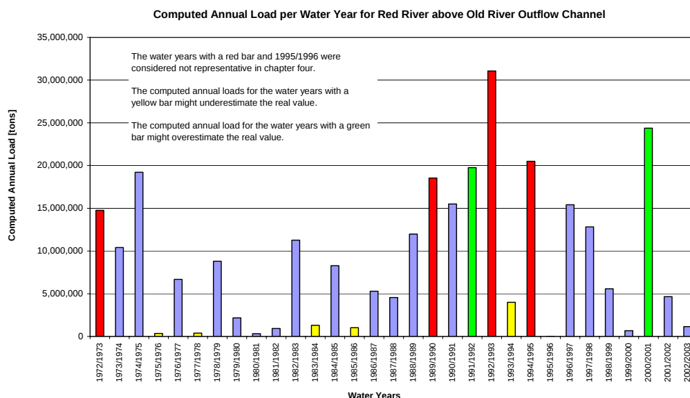
Figure 7 Computed Annual Load per Water Year for Red River above Old River Outflow Channel
