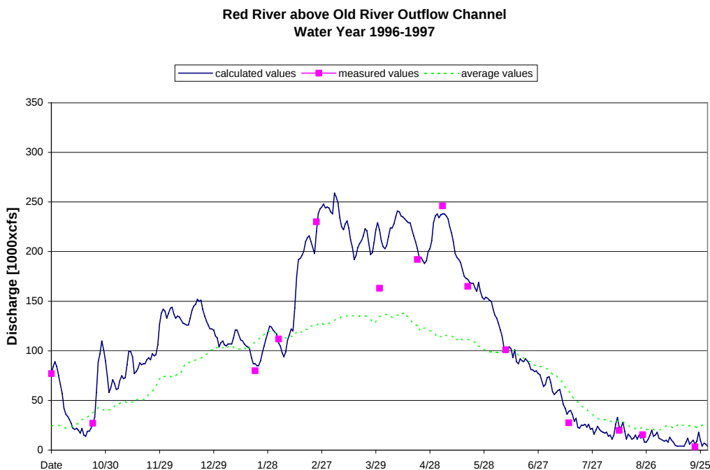
Figure 5 Discharge Graph for the Water Year 1996-1997 at Red River above Old River Outflow Channel, including Calculated and Measured Discharge Values
