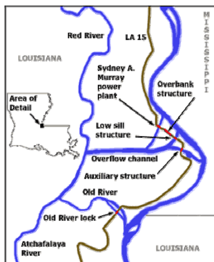
Figure 1 Old River Control Complex
