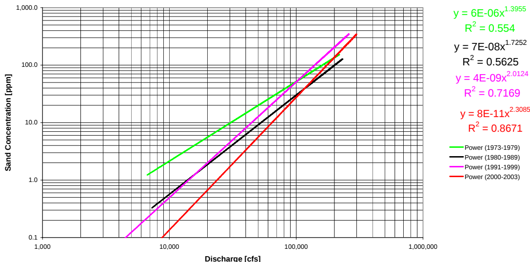
Figure 6 Combined Discharge-Sand Concentration Graph for Red River above Old River Outflow Channel
