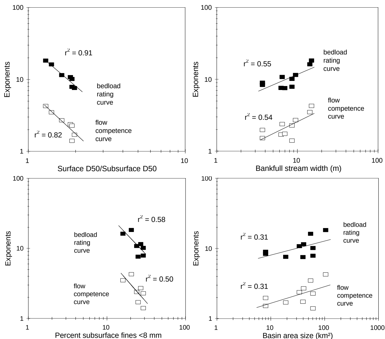
Figure 3 Relationship of exponents of bedload rating and flow competence curves with streambed and stream size parameters.
