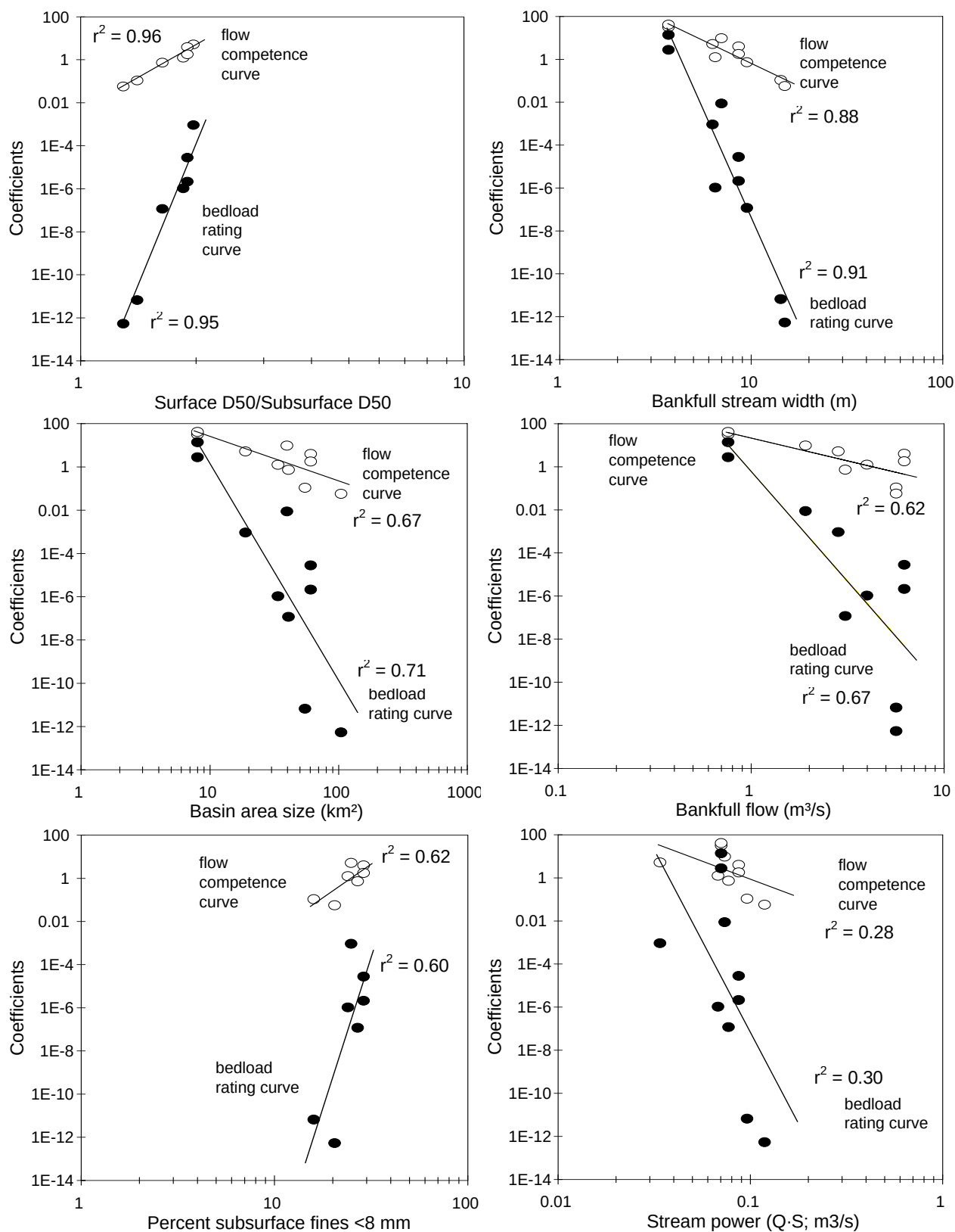
Figure 4 Relationship of the bedload rating and flow competence curve coefficients with streambed and stream size parameters.
