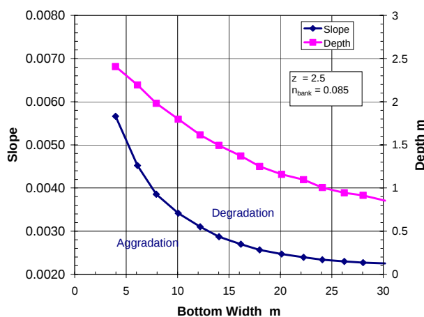
Figure 6 Slope-width-depth family of curves for project.
