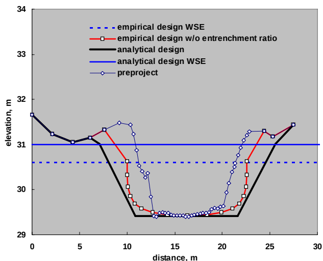
Figure 7 Cross sections for preproject conditions and empirical and analytical designs, White Marsh Run, Maryland.
