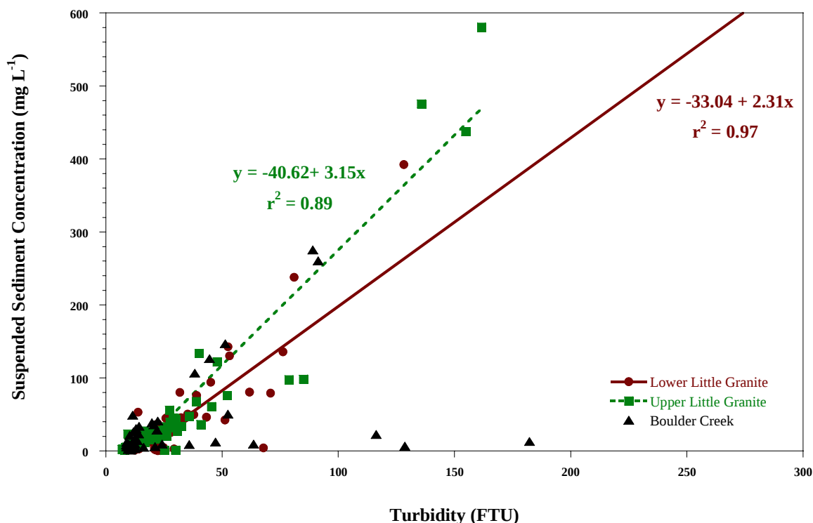
Figure 3 Relationships between turbidity values and measured SSC at 3 sites in Little Granite Creek watershed. Standard error of the residuals at Lower Little Granite was 30.1 and was 33.9 at Upper Little Granite. One additional data point for Lower Little Granite is beyond the limits of this plot, but is included in the regression. No single regression could be determined for the Boulder Creek site as the relationship between turbidity and SSC varied over the measurement period.
