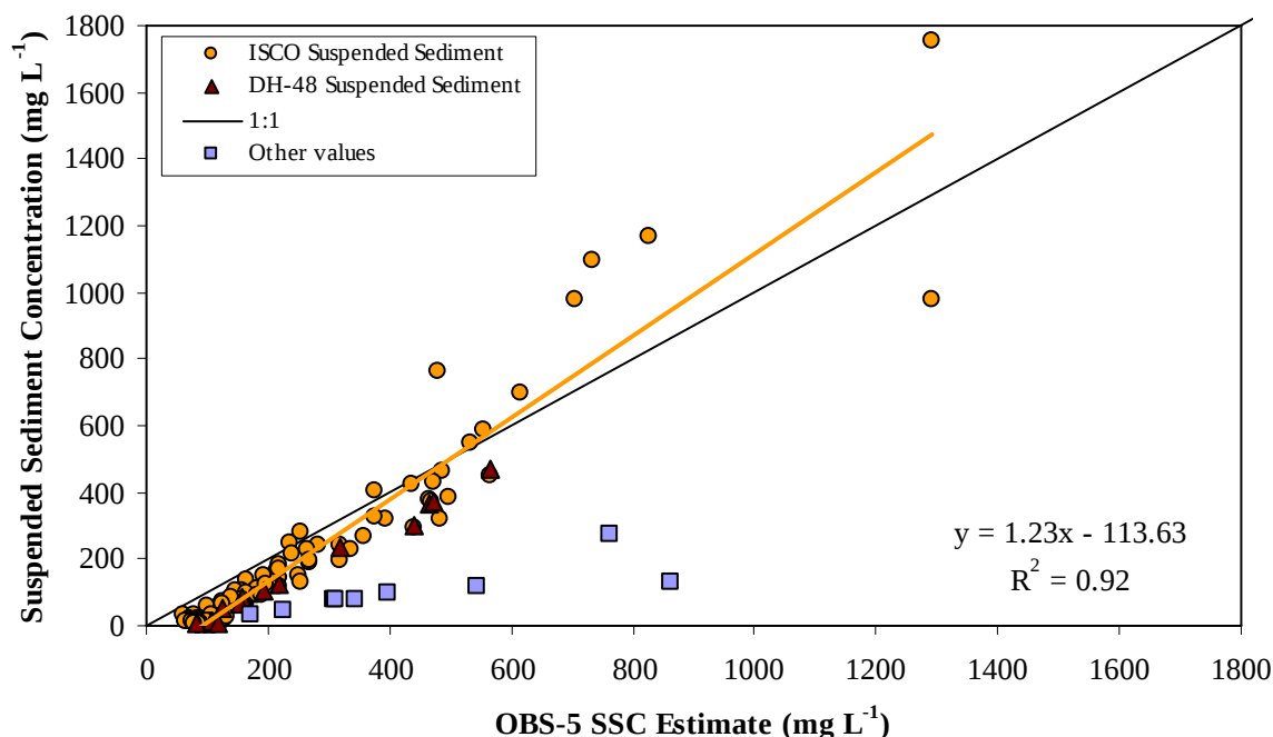
Figure 2 Relationship between estimates of suspended sediment concentration obtained with a (calibrated) OBS-5 turbidity sensor and measurements from ISCO automated samplers (orange circles) at Lower Little Granite Creek. Correspondence between samples obtained with automated and depth-integrated samplers was close to 1:1, as shown by the overlap between orange circles (ISCO) and red triangles (DH-48). This indicates that the flow was well-mixed and no correction factor for the automated sampler was required. Purple squares (excluded from the regression) depict a drift in the relationship between turbidity and ISCO samples following a rain storm in late summer.
