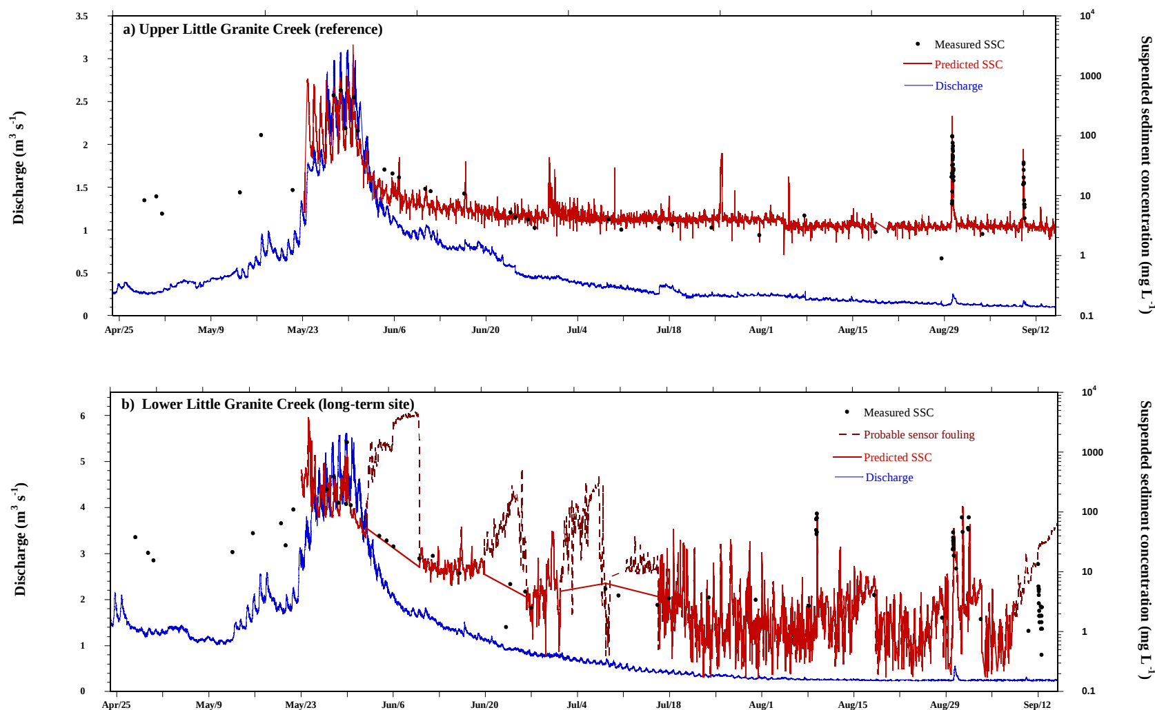
Figure 4 Suspended sediment concentration estimated from values of turbidity from OBS-3 sensors at a) Upper and b) Lower Little Granite Creeks in 2003 (red line). Individual DH-48 samples are shown as black circles and discharge is indicated as a blue line. SSC is plotted on a logarithmic scale to show better the correspondence between predicted and measured values. Though a slightly larger range of values exists for Lower Little Granite during baseflow, this appears exaggerated in (b) where the values cross more than 1 log cycle.
