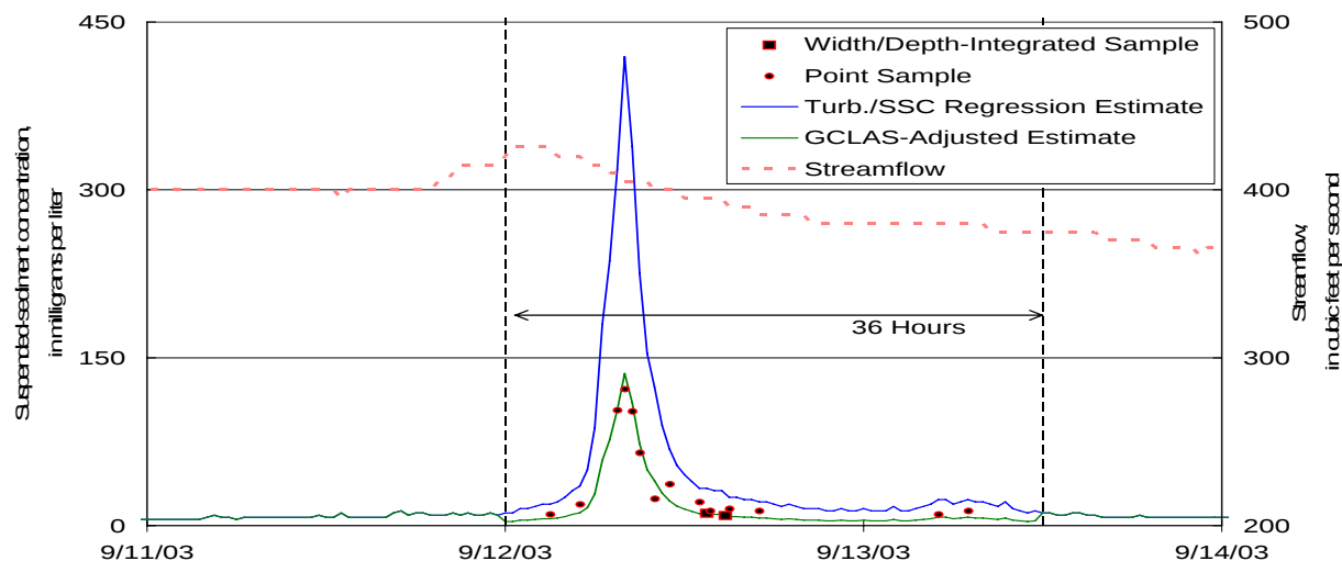
Figure 5 Adjustment of estimated suspended-sediment concentrations for September 2003.
