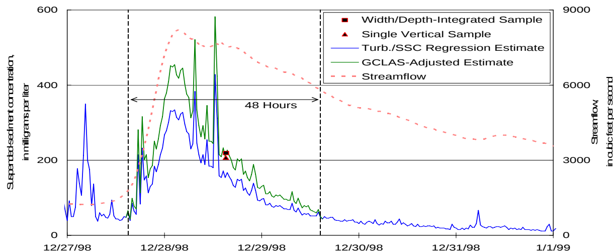
Figure 4 Adjustment of estimated suspended-sediment concentrations for December 27-29, 1998.
