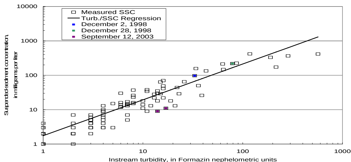
Figure 2 Turbidity and suspended-sediment concentration regression line
