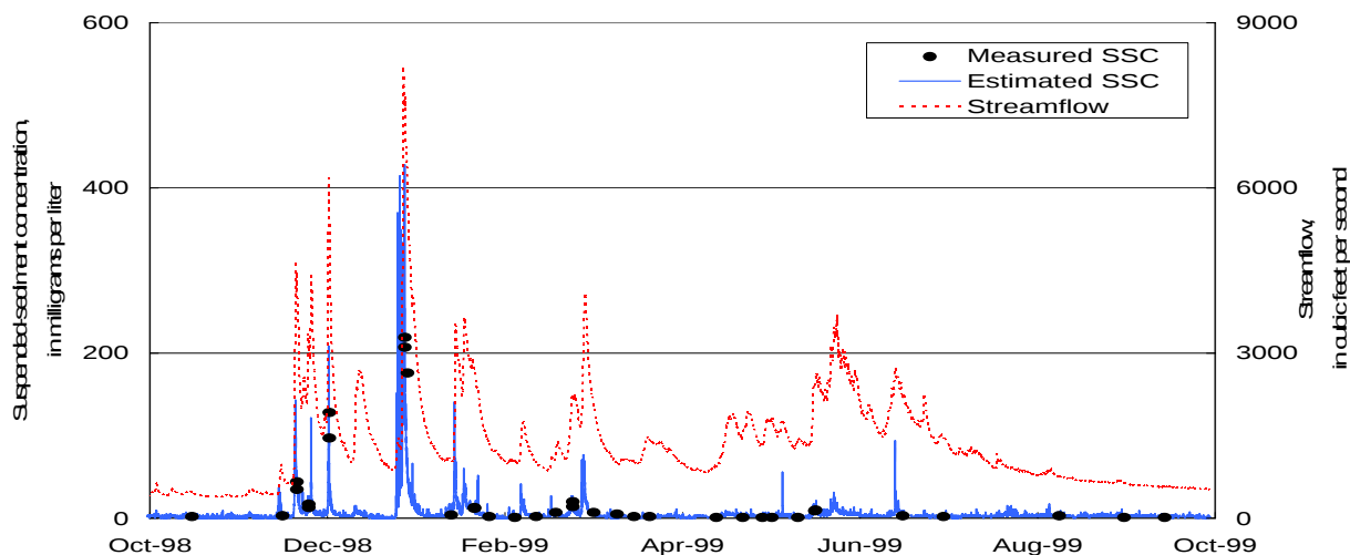
Figure 1 Instantaneous streamflow, measured SSC and estimated SSC, North Santiam River above Boulder Creek, 1999 water year
