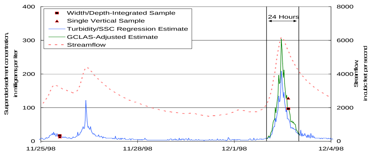
Figure 3 Adjustment of estimated suspended-sediment concentrations for December 2, 1998.
